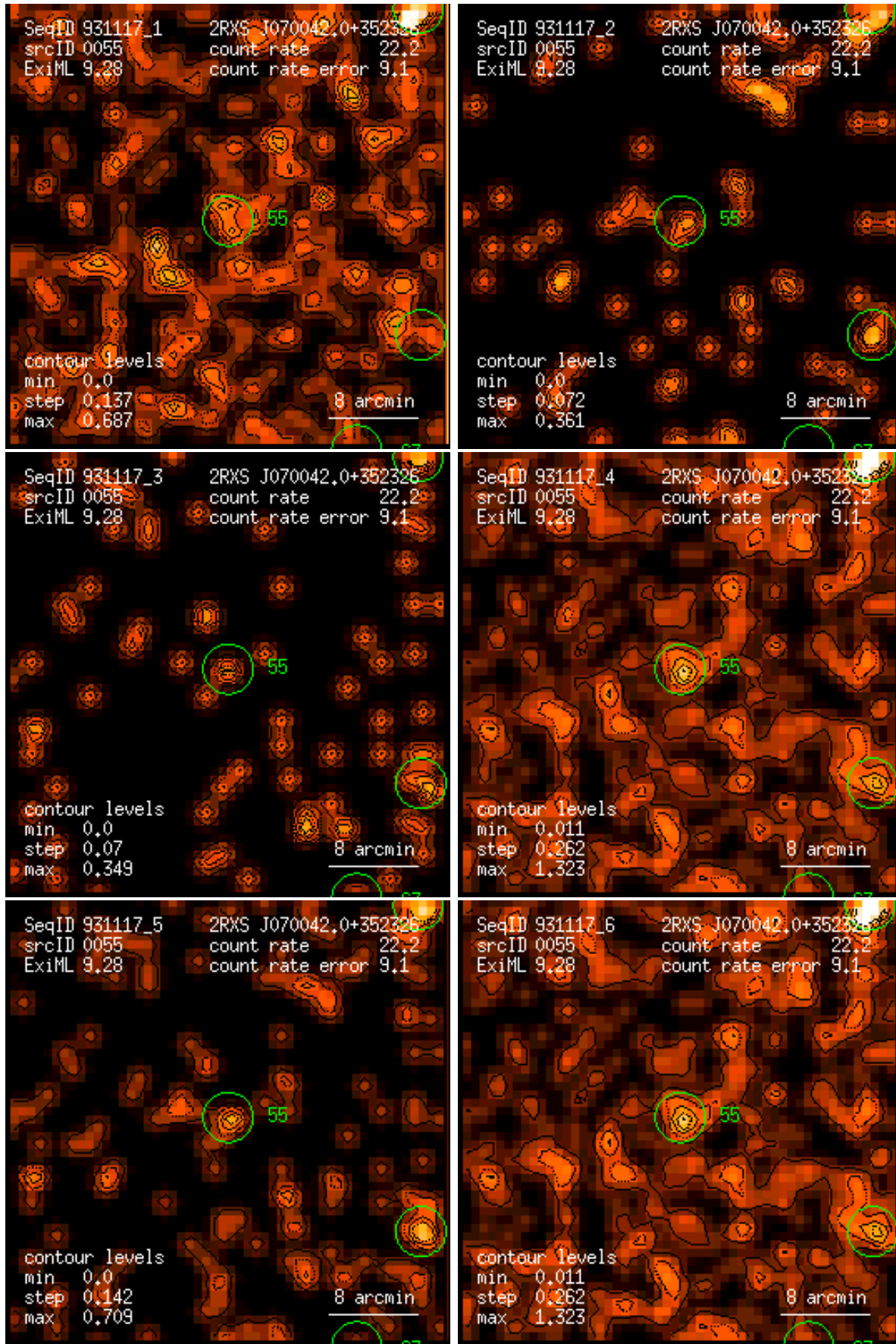
Figure 55: RASS 931117: detection 0055: band rate images, Gaussian filter: (1) PSPC channels 11 – 41, (2) 52 – 90, (3) 91 – 201, (4) 11 – 235, (5) 52 – 201, (6) 11 – 201. Broad band rates in counts/ks. Band rate contour levels in counts/ks/arcmin 2 .
