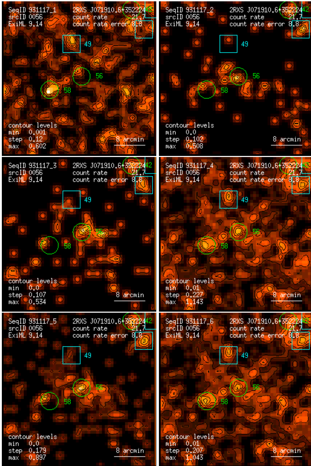
Figure 56: RASS 931117: detection 0056: band rate images, Gaussian filter: (1) PSPC channels 11 – 41, (2) 52 – 90, (3) 91 – 201, (4) 11 – 235, (5) 52 – 201, (6) 11 – 201. Broad band rates in counts/ks. Band rate contour levels in counts/ks/arcmin 2 .
