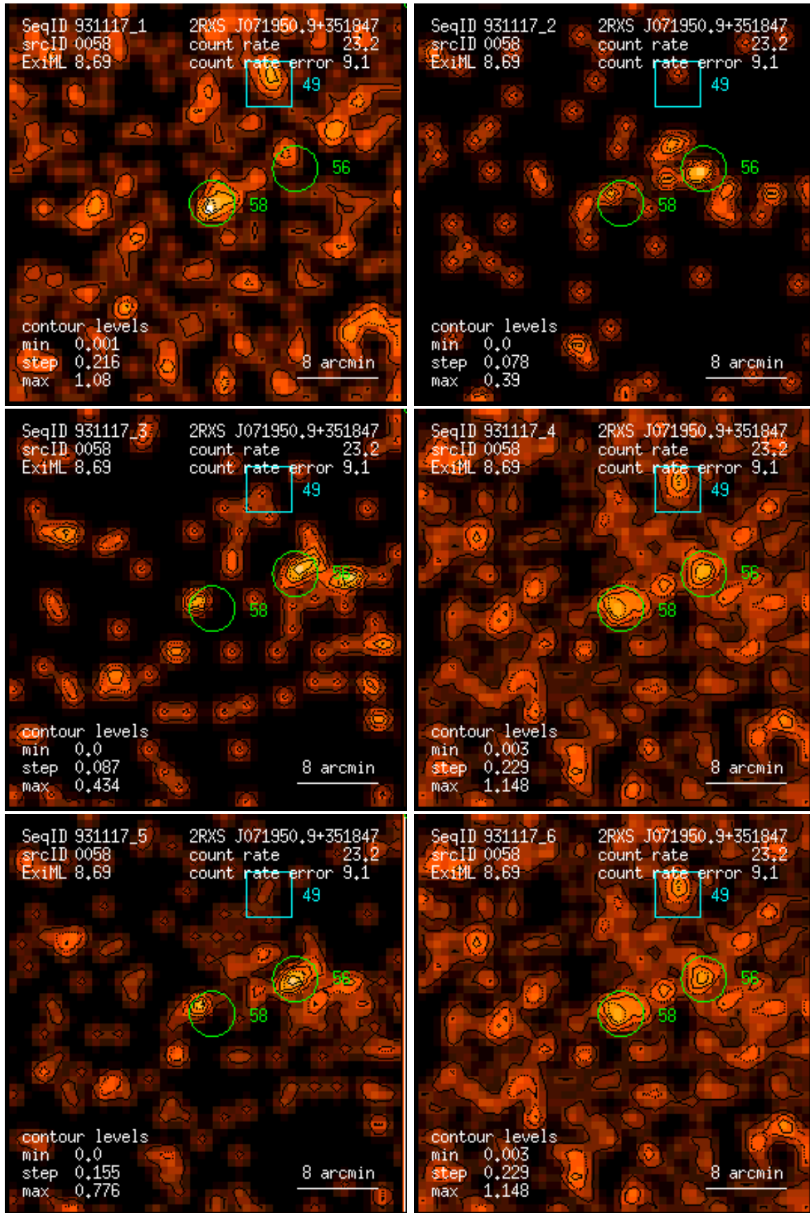
Figure 58: RASS 931117: detection 0058: band rate images, Gaussian filter: (1) PSPC channels 11 – 41, (2) 52 – 90, (3) 91 – 201, (4) 11 – 235, (5) 52 – 201, (6) 11 – 201. Broad band rates in counts/ks. Band rate contour levels in counts/ks/arcmin 2 .
