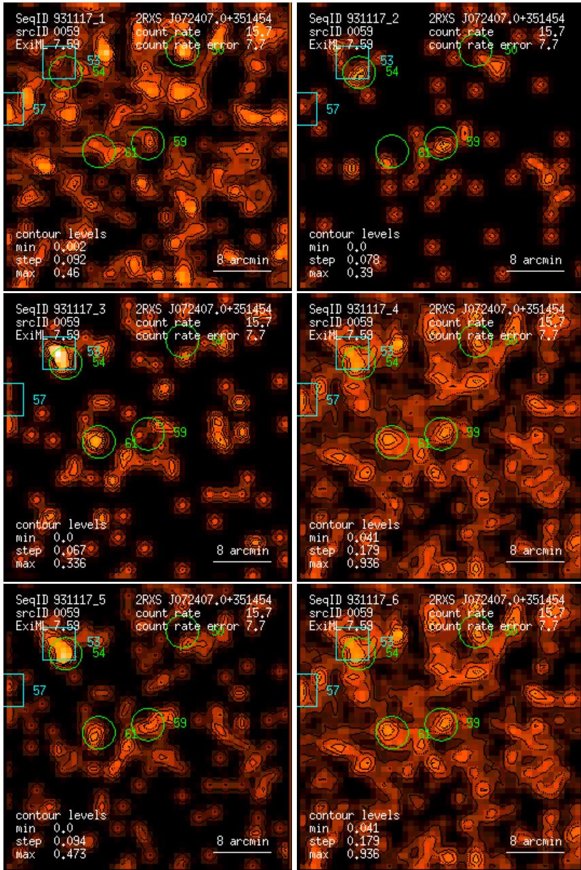
Figure 59: RASS 931117: detection 0059: band rate images, Gaussian filter: (1) PSPC channels 11 – 41, (2) 52 – 90, (3) 91 – 201, (4) 11 – 235, (5) 52 – 201, (6) 11 – 201. Broad band rates in counts/ks. Band rate contour levels in counts/ks/arcmin 2 .
