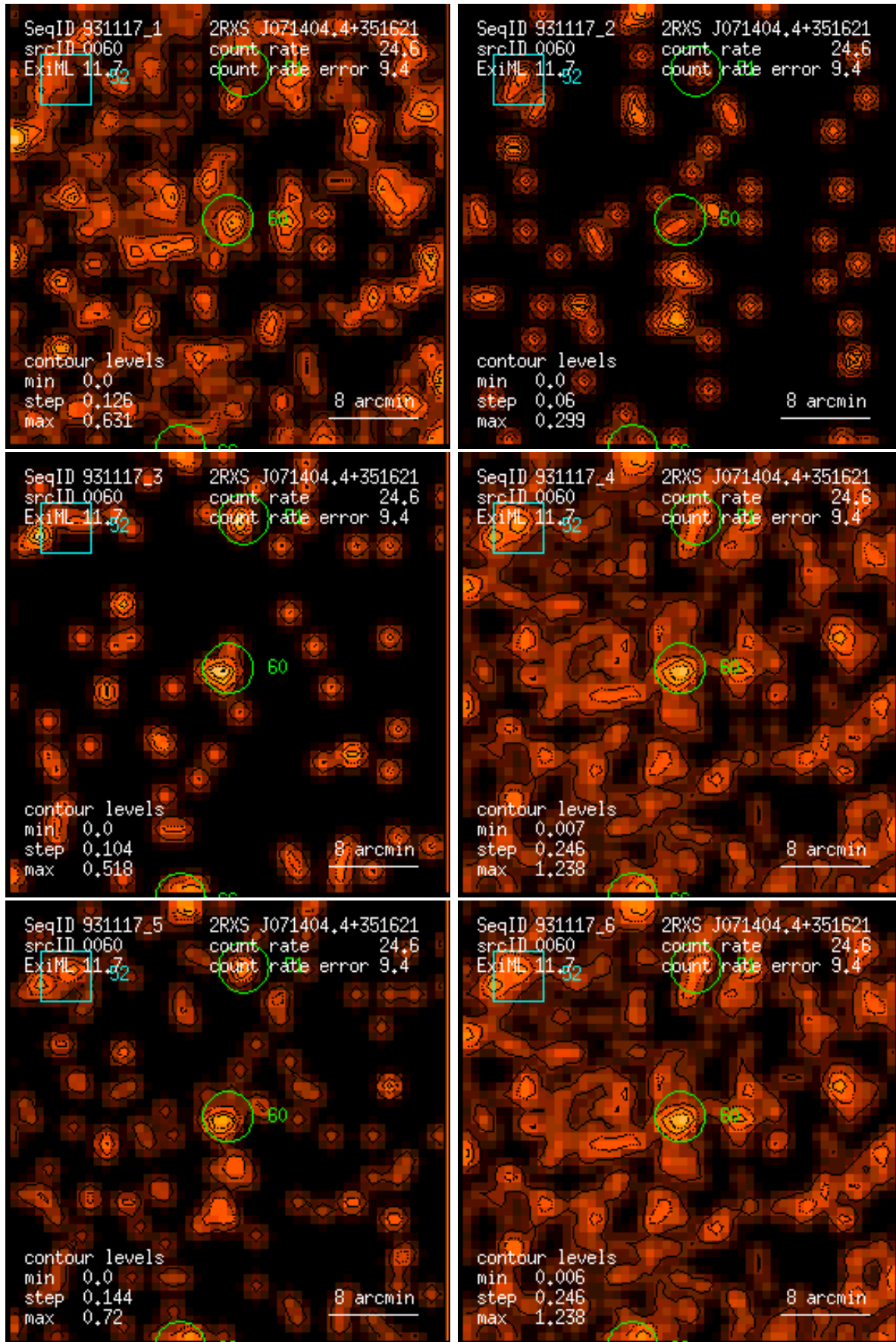
Figure 60: RASS 931117: detection 0060: band rate images, Gaussian filter: (1) PSPC channels 11 – 41, (2) 52 – 90, (3) 91 – 201, (4) 11 – 235, (5) 52 – 201, (6) 11 – 201. Broad band rates in counts/ks. Band rate contour levels in counts/ks/arcmin 2 .
