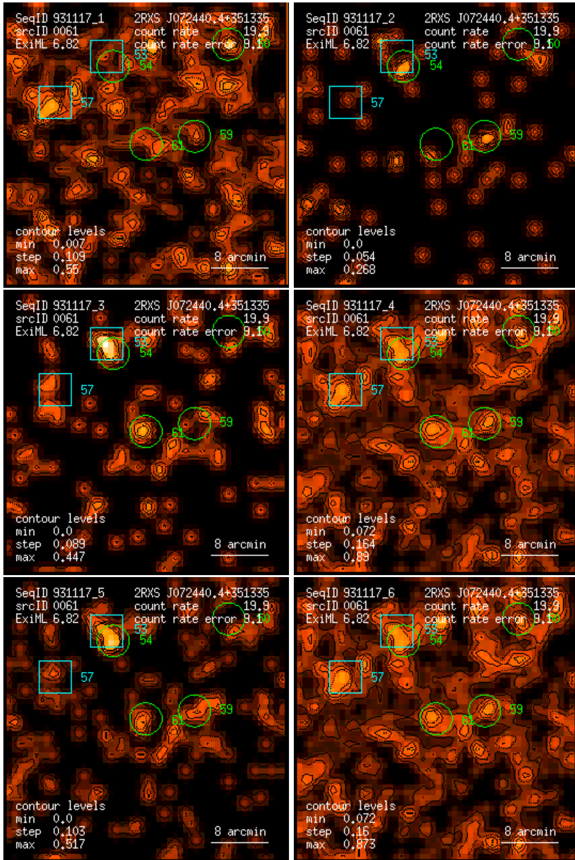
Figure 61: RASS 931117: detection 0061: band rate images, Gaussian filter: (1) PSPC channels 11 – 41, (2) 52 – 90, (3) 91 – 201, (4) 11 – 235, (5) 52 – 201, (6) 11 – 201. Broad band rates in counts/ks. Band rate contour levels in counts/ks/arcmin 2 .
