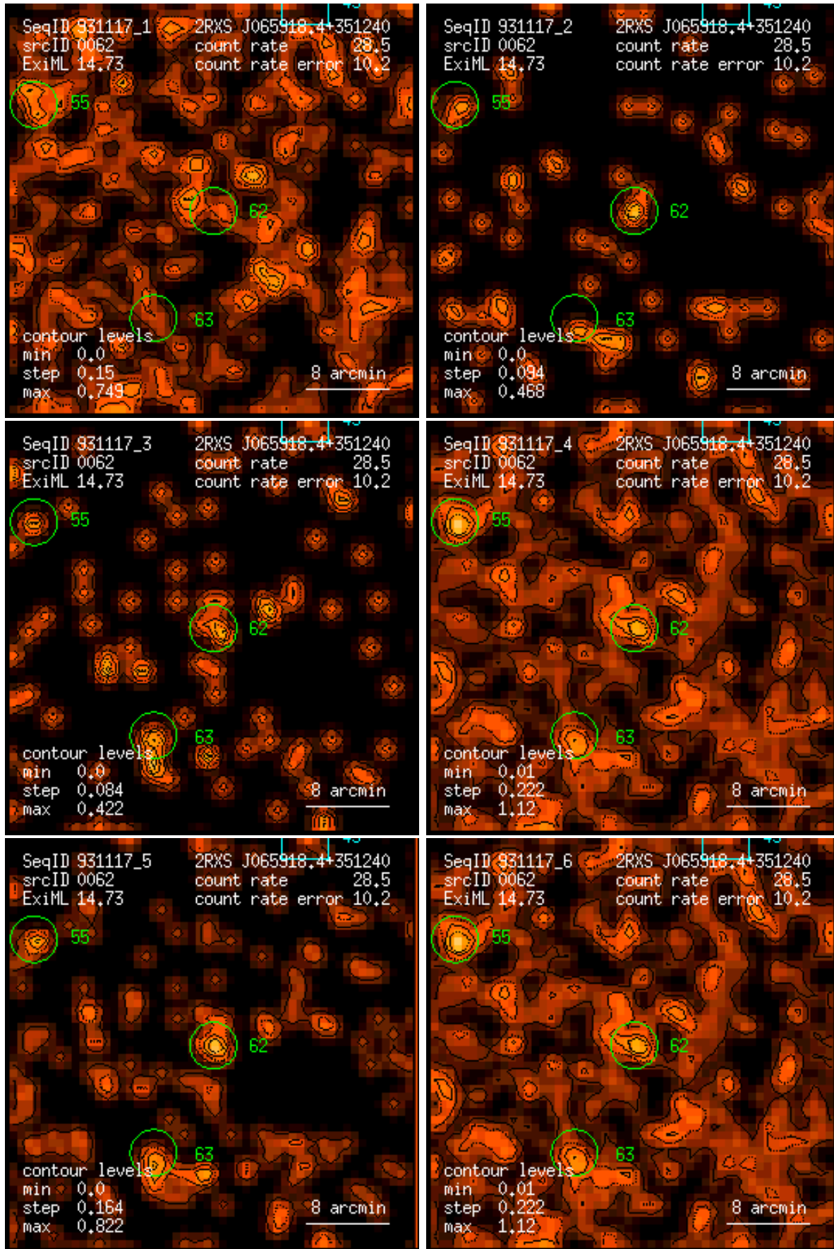
Figure 62: RASS 931117: detection 0062: band rate images, Gaussian filter: (1) PSPC channels 11 – 41, (2) 52 – 90, (3) 91 – 201, (4) 11 – 235, (5) 52 – 201, (6) 11 – 201. Broad band rates in counts/ks. Band rate contour levels in counts/ks/arcmin 2 .
