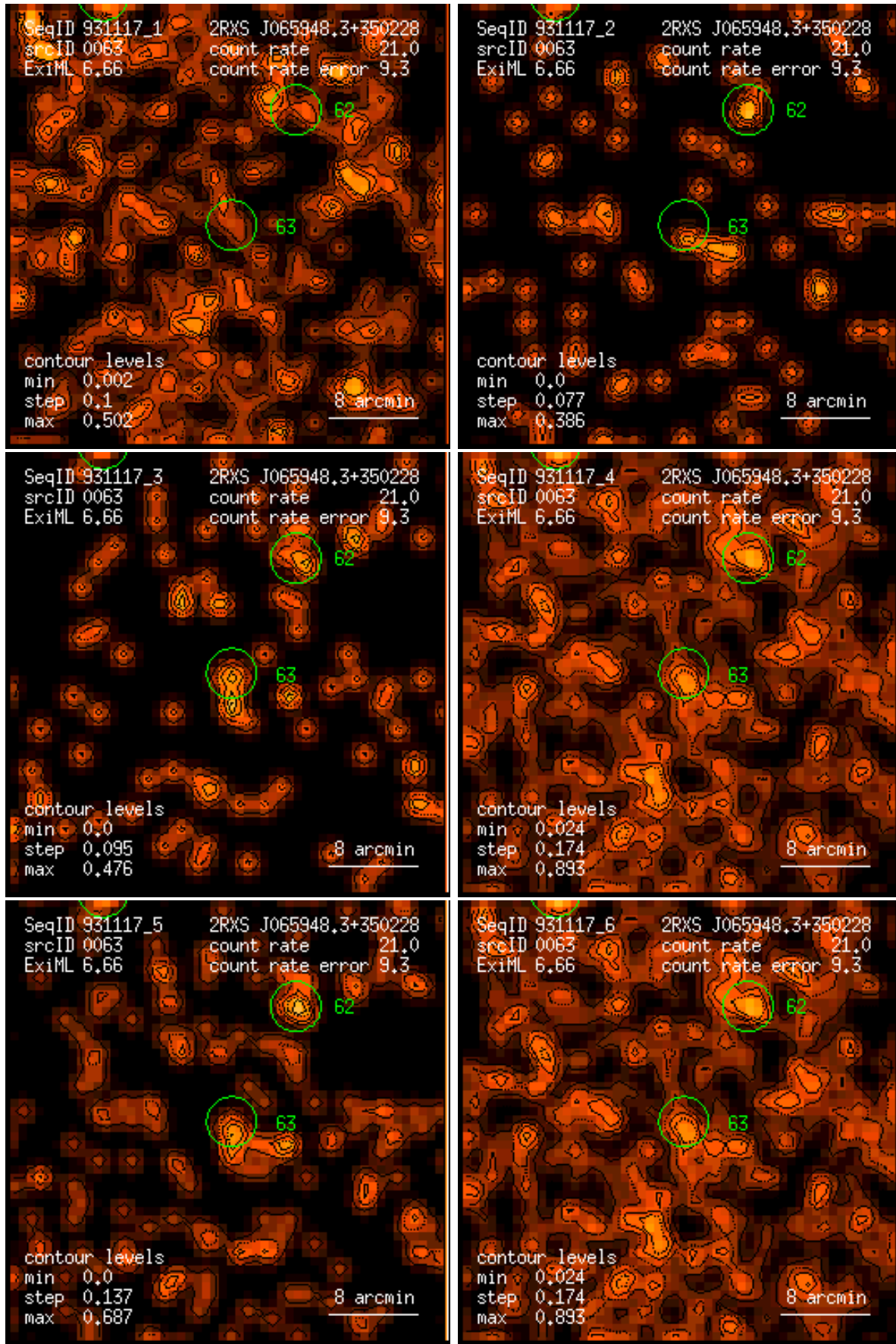
Figure 63: RASS 931117: detection 0063: band rate images, Gaussian filter: (1) PSPC channels 11 – 41, (2) 52 – 90, (3) 91 – 201, (4) 11 – 235, (5) 52 – 201, (6) 11 – 201. Broad band rates in counts/ks. Band rate contour levels in counts/ks/arcmin 2 .
