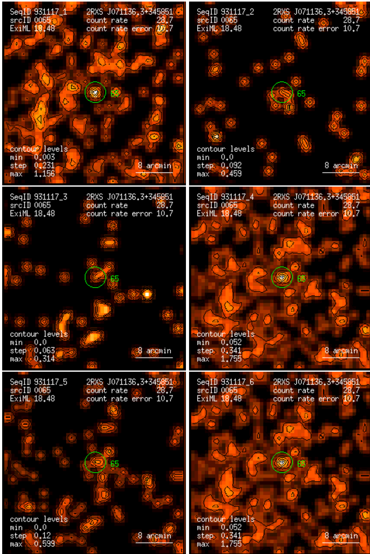
Figure 65: RASS 931117: detection 0065: band rate images, Gaussian filter: (1) PSPC channels 11 – 41, (2) 52 – 90, (3) 91 – 201, (4) 11 – 235, (5) 52 – 201, (6) 11 – 201. Broad band rates in counts/ks. Band rate contour levels in counts/ks/arcmin 2 .
