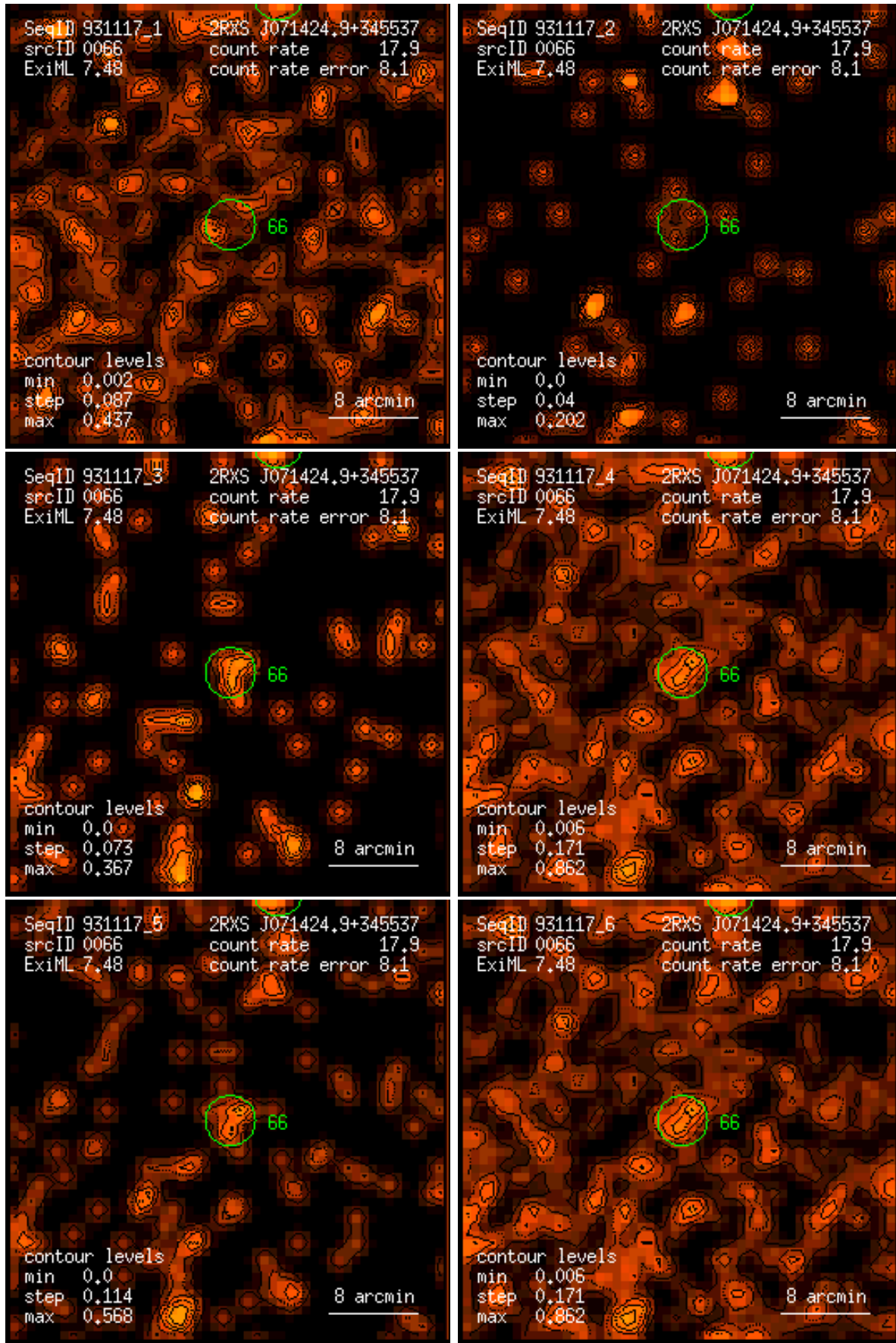
Figure 66: RASS 931117: detection 0066: band rate images, Gaussian filter: (1) PSPC channels 11 – 41, (2) 52 – 90, (3) 91 – 201, (4) 11 – 235, (5) 52 – 201, (6) 11 – 201. Broad band rates in counts/ks. Band rate contour levels in counts/ks/arcmin 2 .
