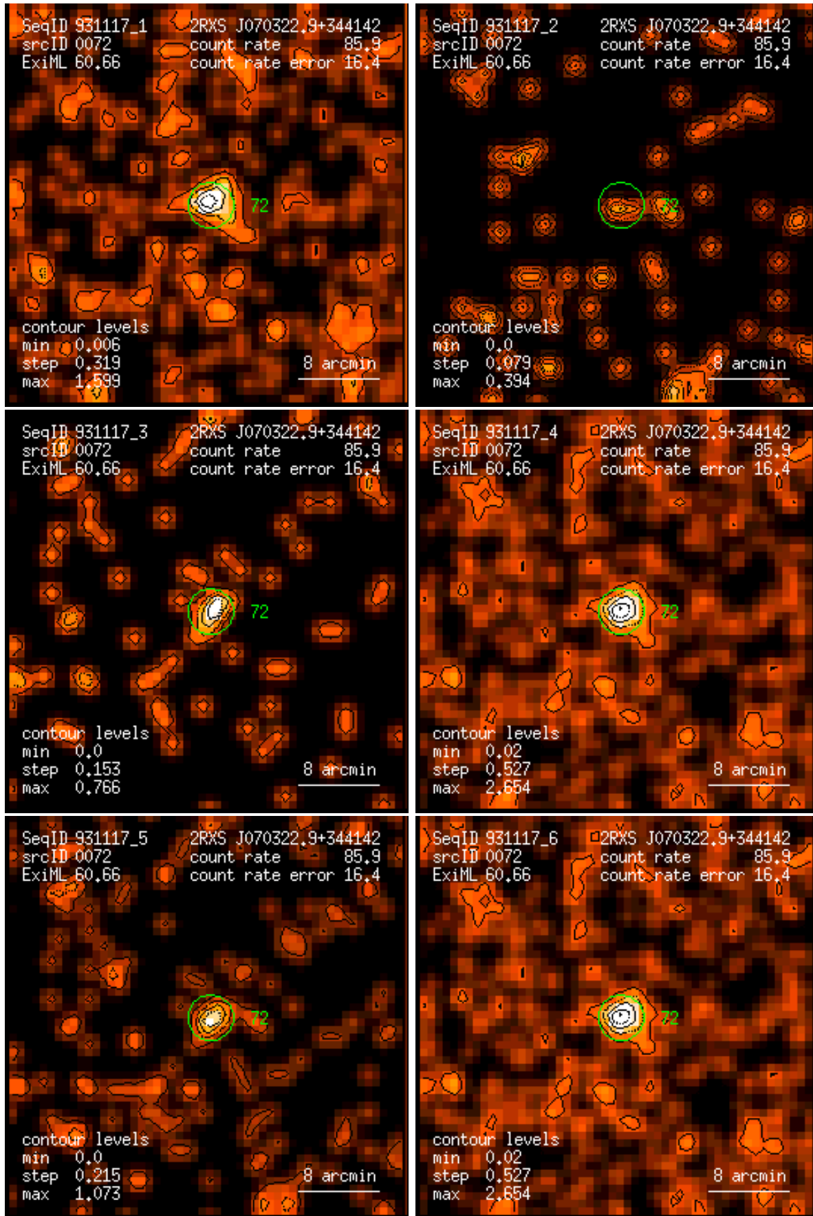
Figure 72: RASS 931117: detection 0072: band rate images, Gaussian filter: (1) PSPC channels 11 – 41, (2) 52 – 90, (3) 91 – 201, (4) 11 – 235, (5) 52 – 201, (6) 11 – 201. Broad band rates in counts/ks. Band rate contour levels in counts/ks/arcmin 2 .
