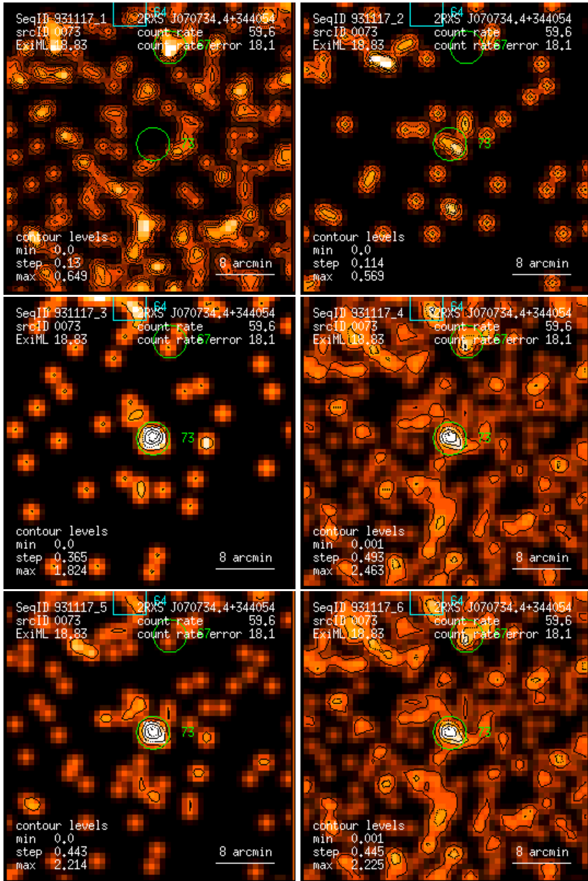
Figure 73: RASS 931117: detection 0073: band rate images, Gaussian filter: (1) PSPC channels 11 – 41, (2) 52 – 90, (3) 91 – 201, (4) 11 – 235, (5) 52 – 201, (6) 11 – 201. Broad band rates in counts/ks. Band rate contour levels in counts/ks/arcmin 2 .
