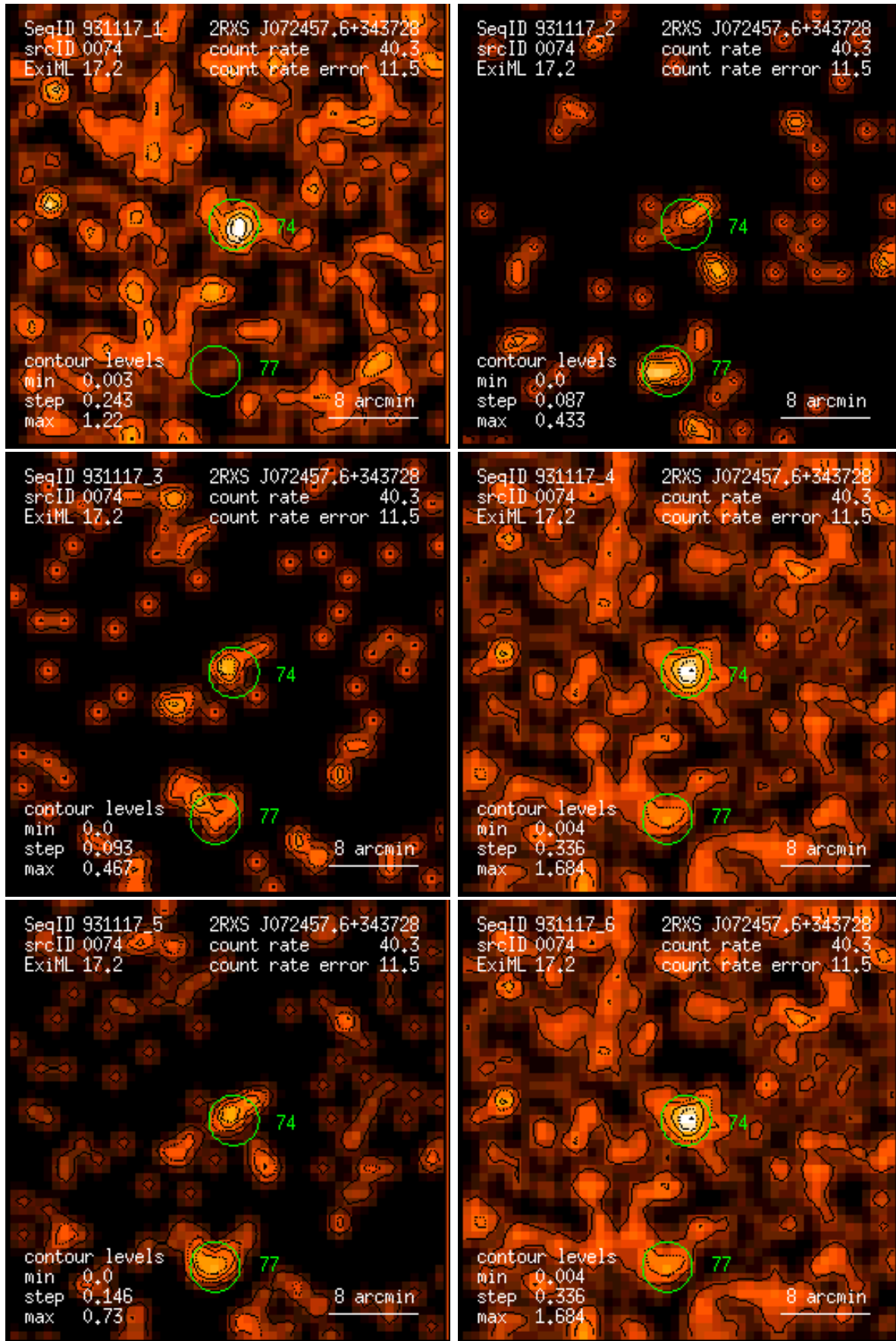
Figure 74: RASS 931117: detection 0074: band rate images, Gaussian filter: (1) PSPC channels 11 – 41, (2) 52 – 90, (3) 91 – 201, (4) 11 – 235, (5) 52 – 201, (6) 11 – 201. Broad band rates in counts/ks. Band rate contour levels in counts/ks/arcmin 2 .
