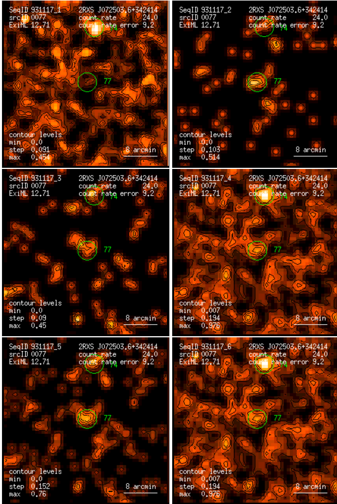
Figure 77: RASS 931117: detection 0077: band rate images, Gaussian filter: (1) PSPC channels 11 – 41, (2) 52 – 90, (3) 91 – 201, (4) 11 – 235, (5) 52 – 201, (6) 11 – 201. Broad band rates in counts/ks. Band rate contour levels in counts/ks/arcmin 2 .
