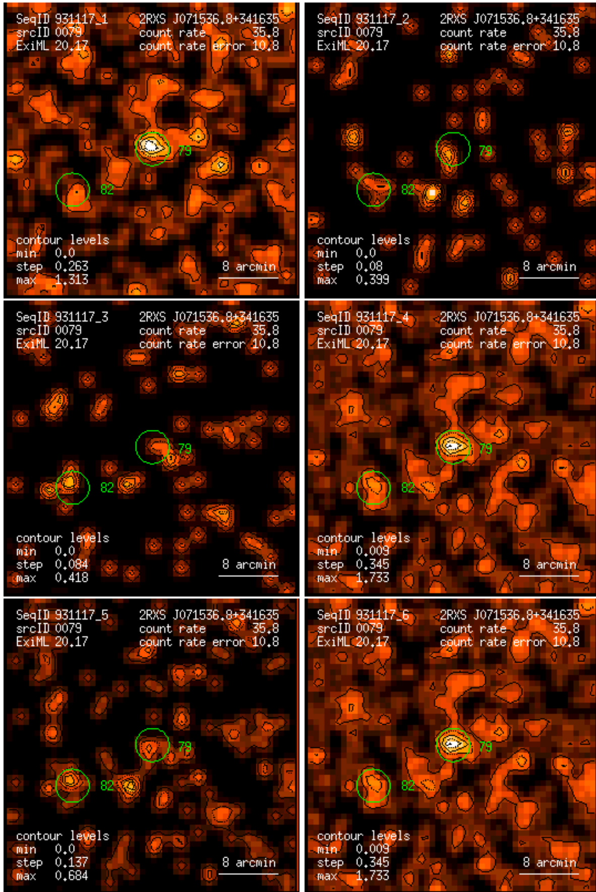
Figure 79: RASS 931117: detection 0079: band rate images, Gaussian filter: (1) PSPC channels 11 – 41, (2) 52 – 90, (3) 91 – 201, (4) 11 – 235, (5) 52 – 201, (6) 11 – 201. Broad band rates in counts/ks. Band rate contour levels in counts/ks/arcmin 2 .
