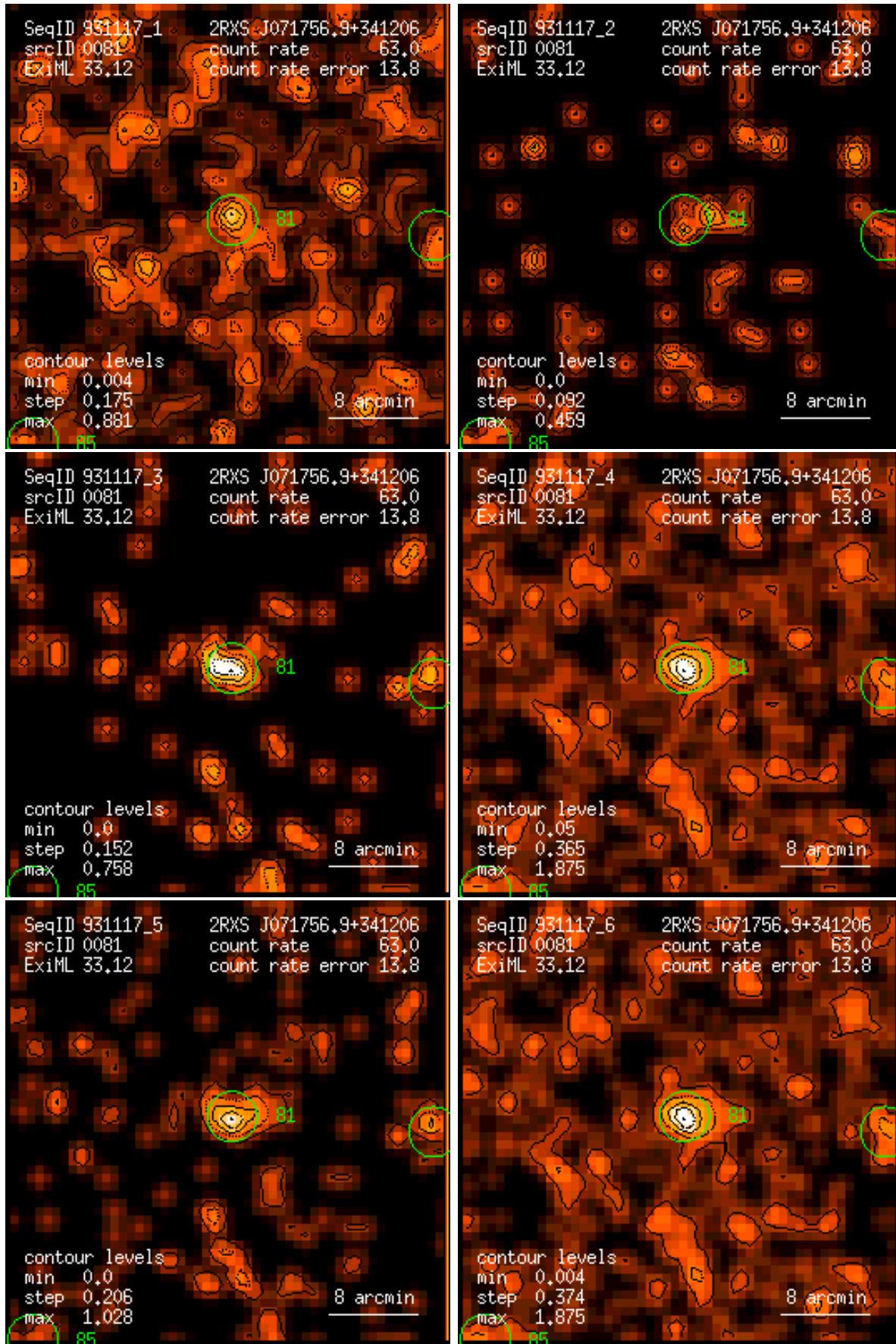
Figure 81: RASS 931117: detection 0081: band rate images, Gaussian filter: (1) PSPP channels 11 – 41, (2) 52 – 90, (3) 91 – 201, (4) 11 – 235, (5) 52 – 201, (6) 11 – 201. Broad band rates in counts/ks. Band rate contour levels in counts/ks/arcmin 2 .
