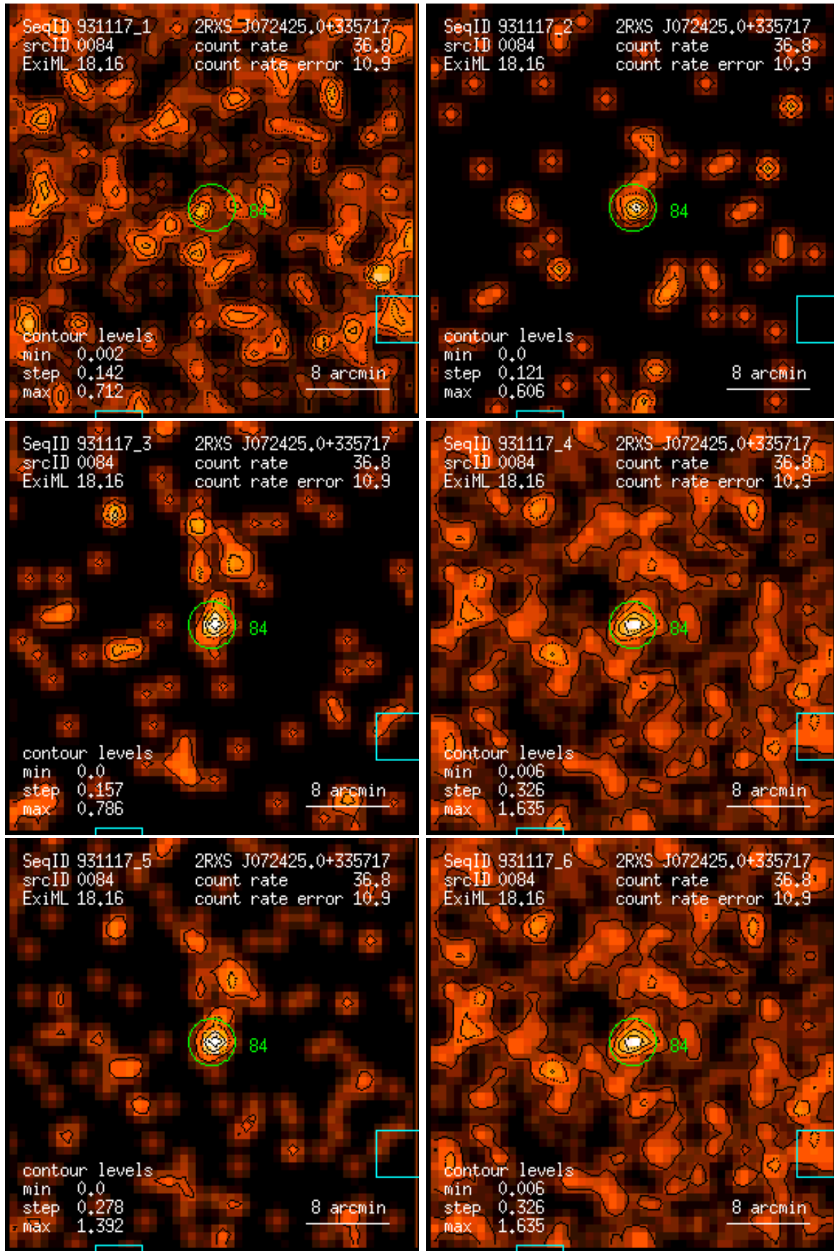
Figure 84: RASS 931117: detection 0084: band rate images, Gaussian filter: (1) PSPC channels 11 – 41, (2) 52 – 90, (3) 91 – 201, (4) 11 – 235, (5) 52 – 201, (6) 11 – 201. Broad band rates in counts/ks. Band rate contour levels in counts/ks/arcmin 2 .
