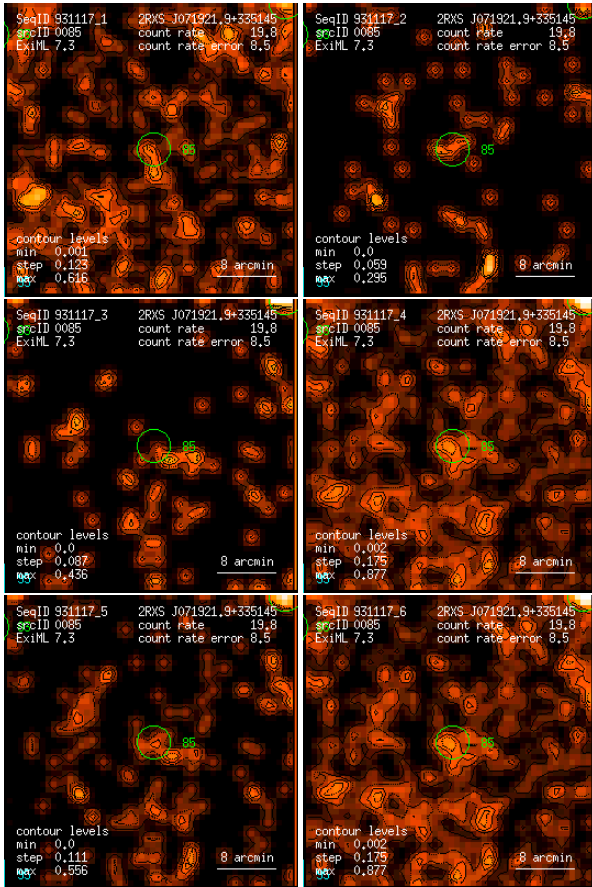
Figure 85: RASS 931117: detection 0085: band rate images, Gaussian filter: (1) PSPC channels 11 – 41, (2) 52 – 90, (3) 91 – 201, (4) 11 – 235, (5) 52 – 201, (6) 11 – 201. Broad band rates in counts/ks. Band rate contour levels in counts/ks/arcmin 2 .
