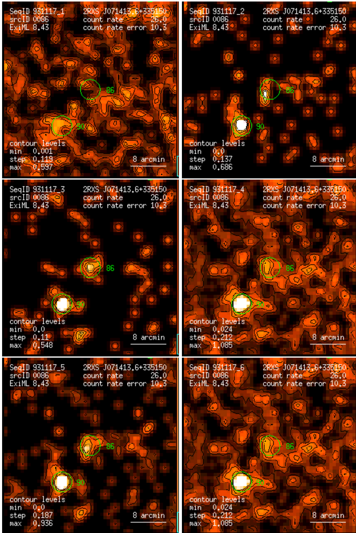
Figure 86: RASS 931117: detection 0086: band rate images, Gaussian filter: (1) PSPC channels 11 – 41, (2) 52 – 90, (3) 91 – 201, (4) 11 – 235, (5) 52 – 201, (6) 11 – 201. Broad band rates in counts/ks. Band rate contour levels in counts/ks/arcmin 2 .
