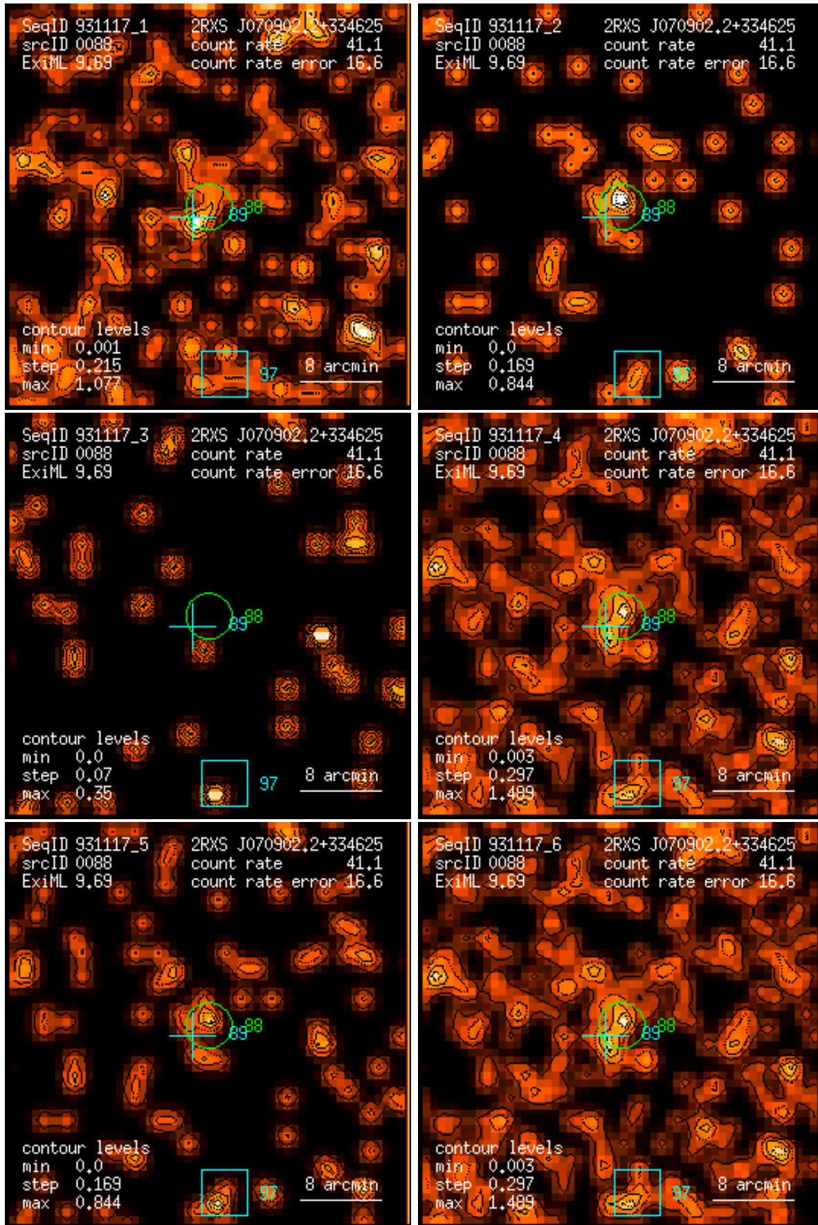
Figure 88: RASS 931117: detection 0088: band rate images, Gaussian filter: (1) PSPC channels 11 – 41, (2) 52 – 90, (3) 91 – 201, (4) 11 – 235, (5) 52 – 201, (6) 11 – 201. Broad band rates in counts/ks. Band rate contour levels in counts/ks/arcmin 2 .
