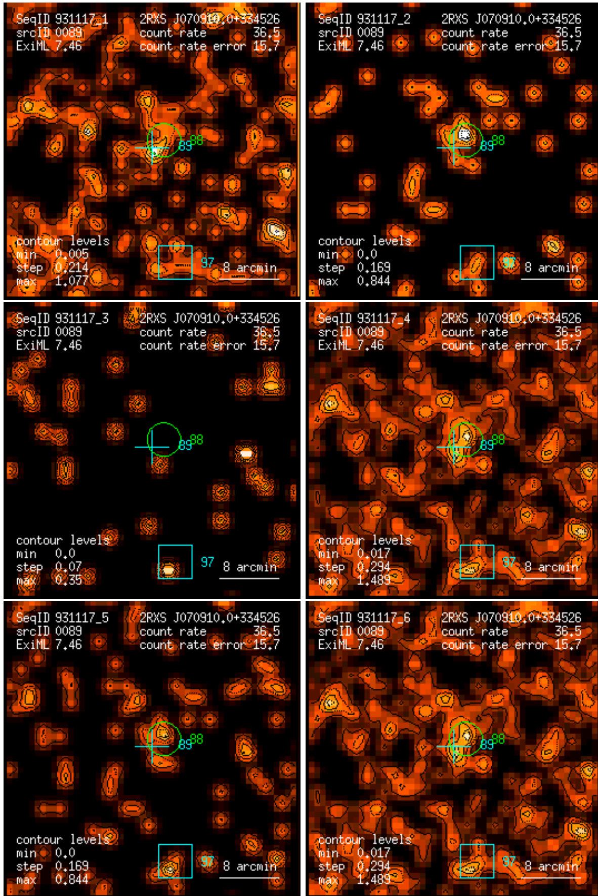
Figure 89: RASS 931117: detection 0089: band rate images, Gaussian filter: (1) PSPC channels 11 – 41, (2) 52 – 90, (3) 91 – 201, (4) 11 – 235, (5) 52 – 201, (6) 11 – 201. Broad band rates in counts/ks. Band rate contour levels in counts/ks/arcmin 2 .
