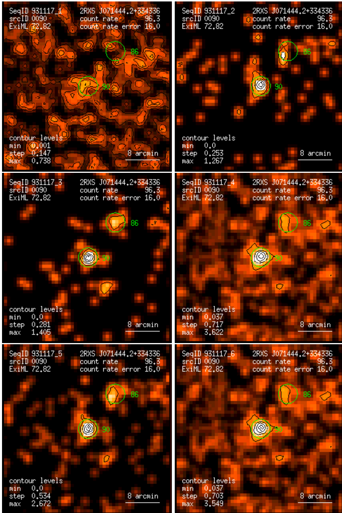
Figure 90: RASS 931117: detection 0090: band rate images, Gaussian filter: (1) PSPC channels 11 – 41, (2) 52 – 90, (3) 91 – 201, (4) 11 – 235, (5) 52 – 201, (6) 11 – 201. Broad band rates in counts/ks. Band rate contour levels in counts/ks/arcmin 2 .
