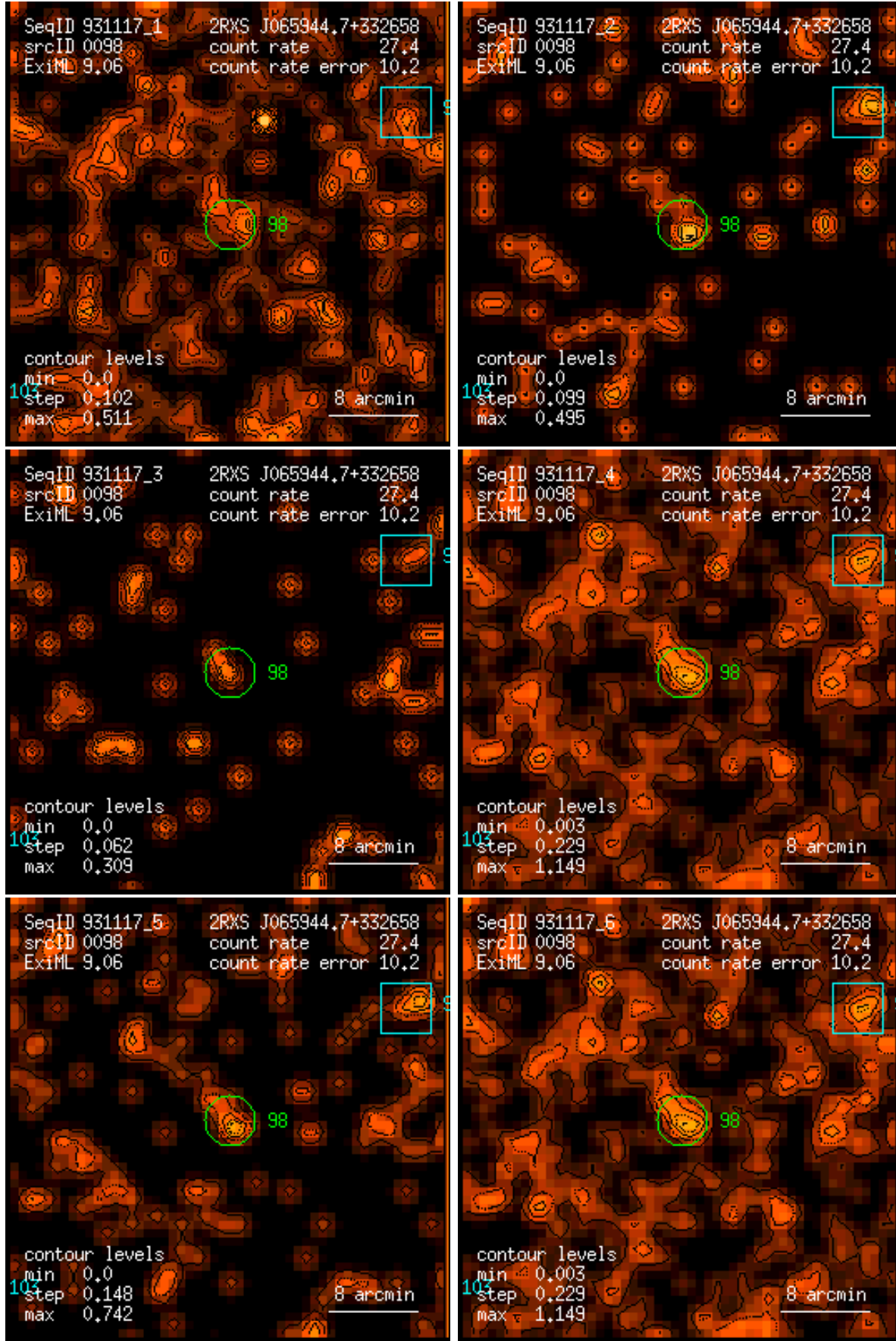
Figure 98: RASS 931117: detection 0098: band rate images, Gaussian filter: (1) PSPC channels 11 – 41, (2) 52 – 90, (3) 91 – 201, (4) 11 – 235, (5) 52 – 201, (6) 11 – 201. Broad band rates in counts/ks. Band rate contour levels in counts/ks/arcmin 2 .
