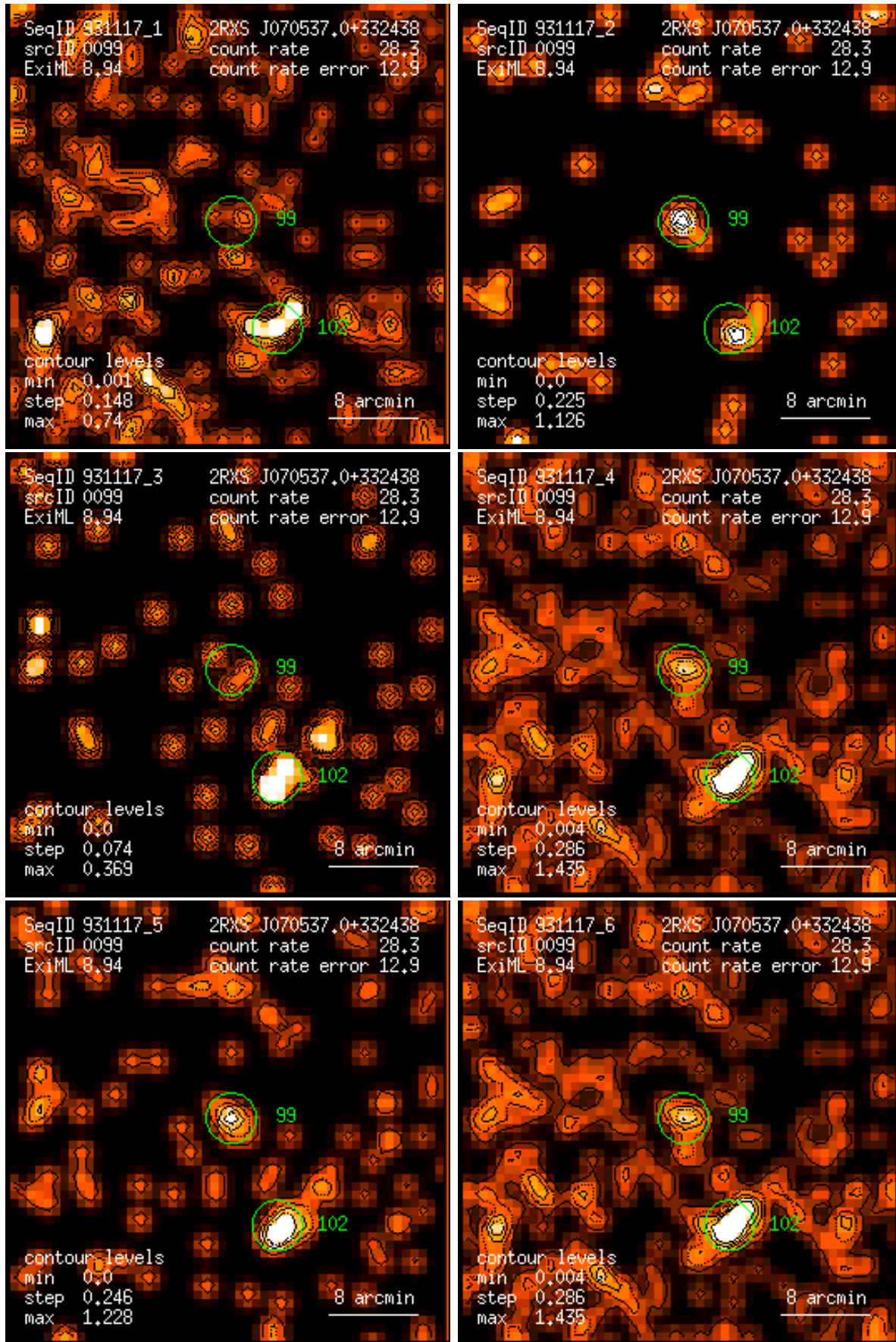
Figure 99: RASS 931117: detection 0099: band rate images, Gaussian filter: (1) PSPC channels 11 – 41, (2) 52 – 90, (3) 91 – 201, (4) 11 – 235, (5) 52 – 201, (6) 11 – 201. Broad band rates in counts/ks. Band rate contour levels in counts/ks/arcmin 2 .
