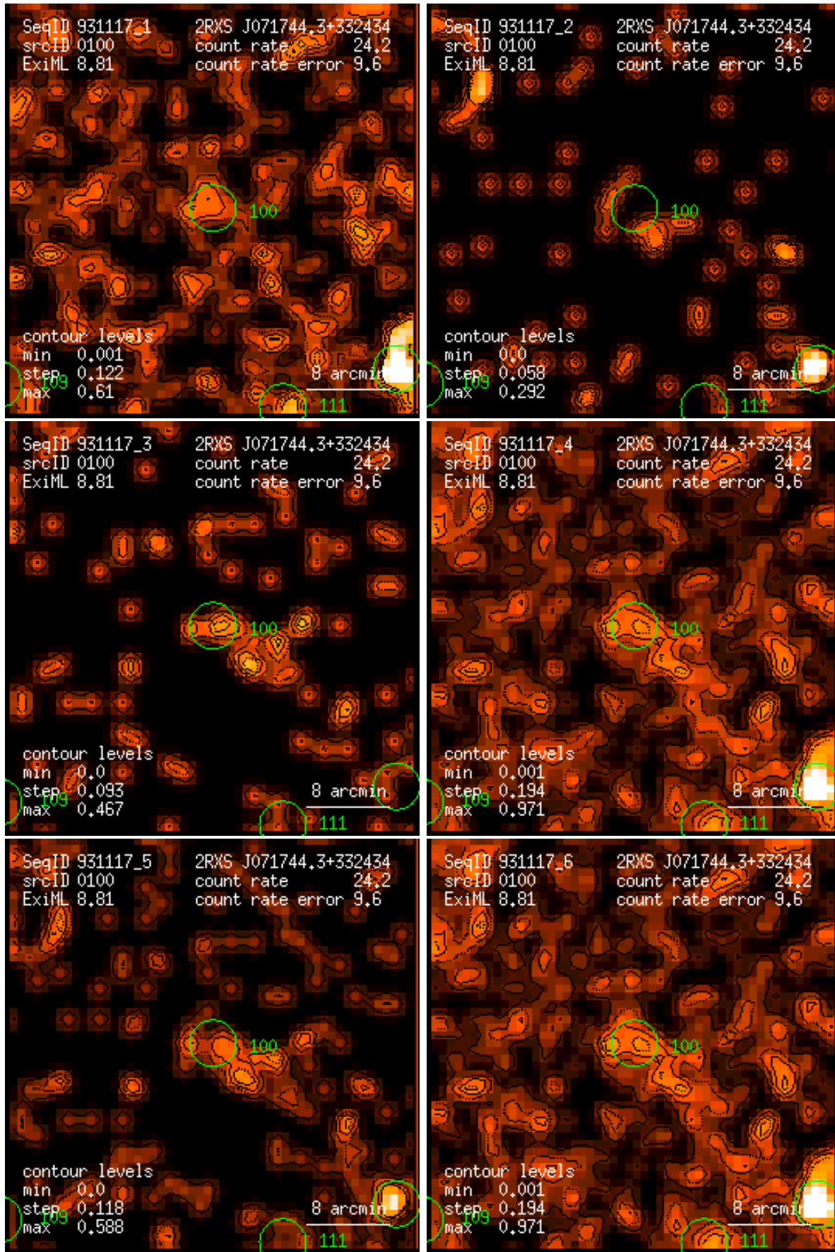
Figure 100: RASS 931117: detection 0100: band rate images, Gaussian filter: (1) PSPC channels 11 – 41, (2) 52 – 90, (3) 91 – 201, (4) 11 – 235, (5) 52 – 201, (6) 11 – 201. Broad band rates in counts/ks. Band rate contour levels in counts/ks/arcmin 2 .
