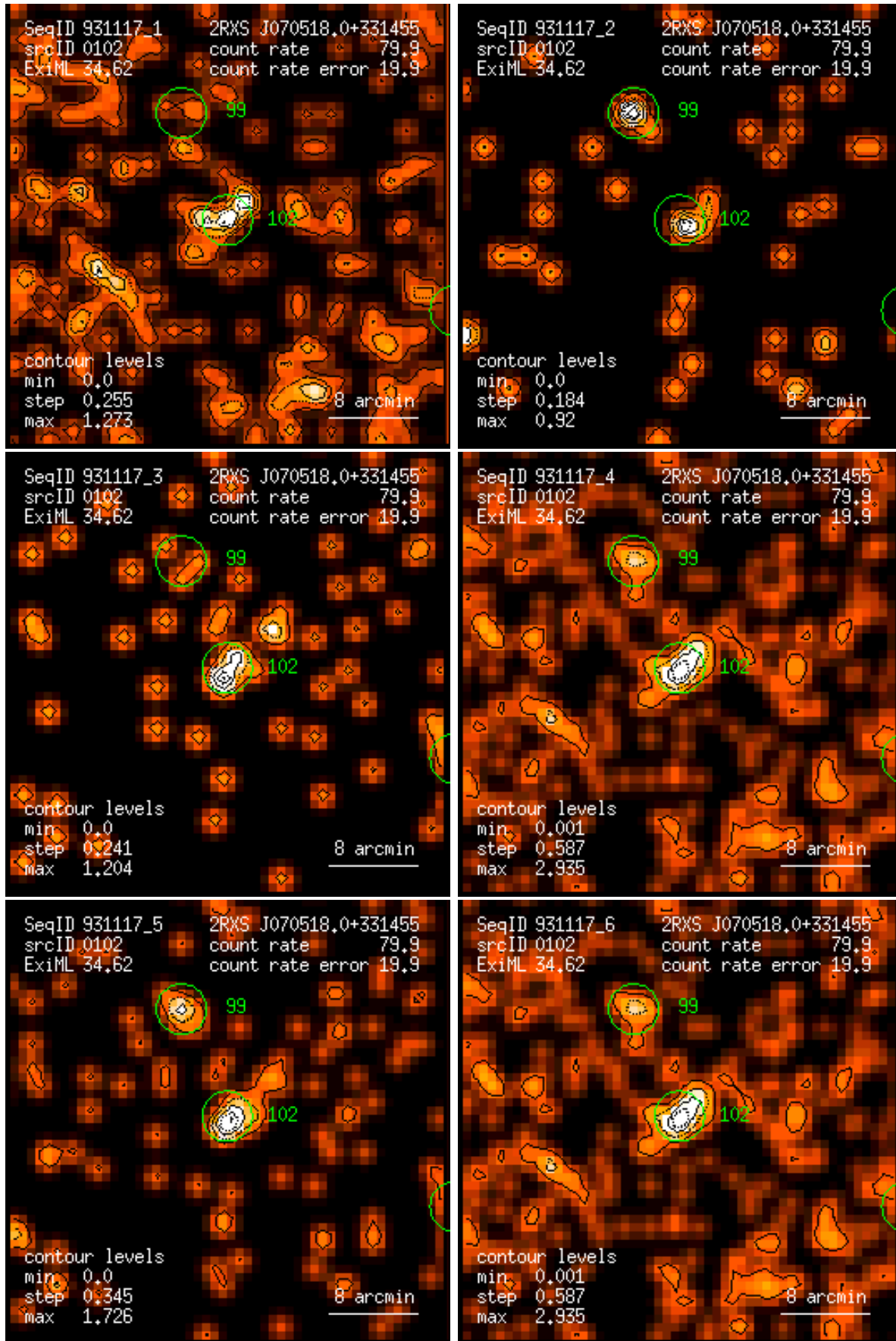
Figure 102: RASS 931117: detection 0102: band rate images, Gaussian filter: (1) PSPC channels 11 – 41, (2) 52 – 90, (3) 91 – 201, (4) 11 – 235, (5) 52 – 201, (6) 11 – 201. Broad band rates in counts/ks. Band rate contour levels in counts/ks/arcmin 2 .
