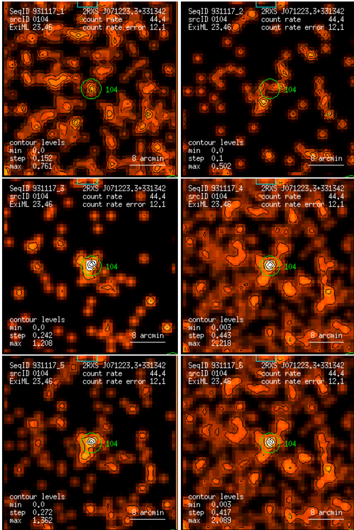
Figure 104: RASS 931117: detection 0104: band rate images, Gaussian filter: (1) PSPC channels 11 – 41, (2) 52 – 90, (3) 91 – 201, (4) 11 – 235, (5) 52 – 201, (6) 11 – 201. Broad band rates in counts/ks. Band rate contour levels in counts/ks/arcmin 2 .
