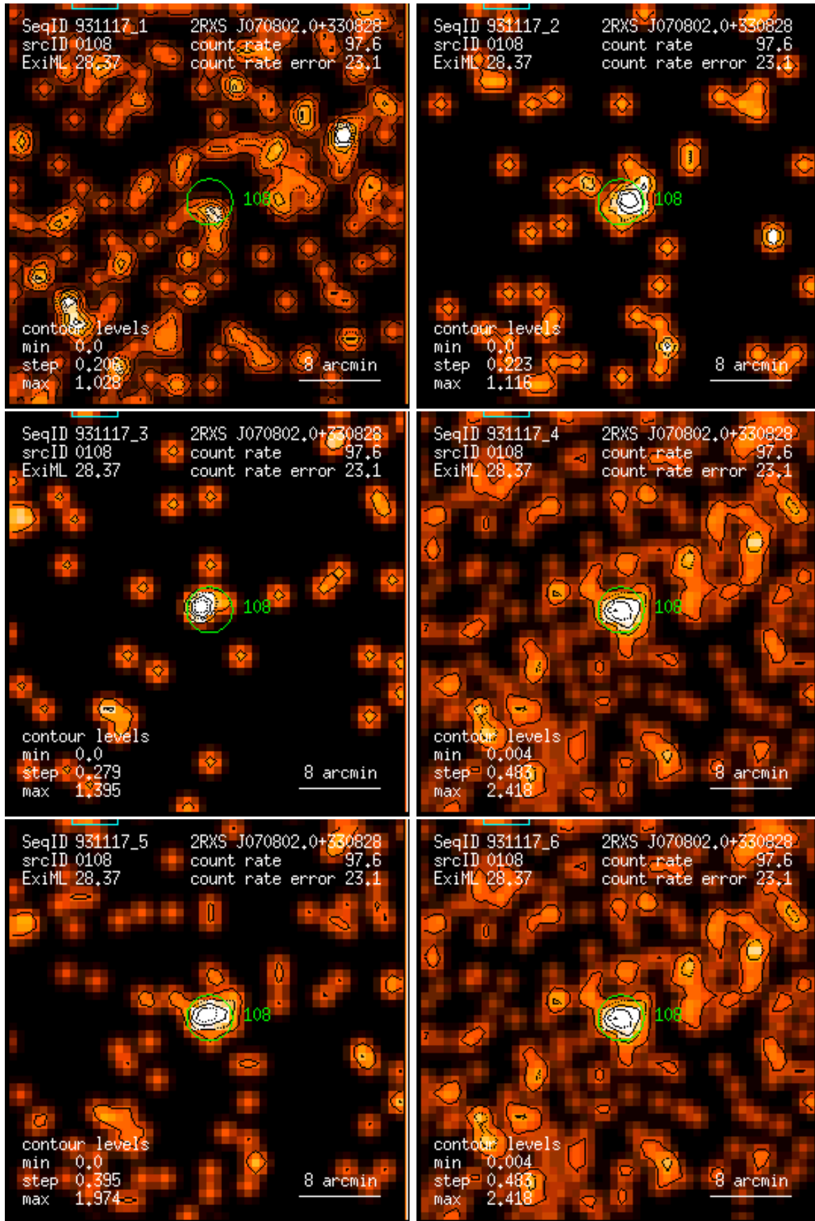
Figure 108: RASS 931117: detection 0108: band rate images, Gaussian filter: (1) PSPC channels 11 – 41, (2) 52 – 90, (3) 91 – 201, (4) 11 – 235, (5) 52 – 201, (6) 11 – 201. Broad band rates in counts/ks. Band rate contour levels in counts/ks/arcmin 2 .
