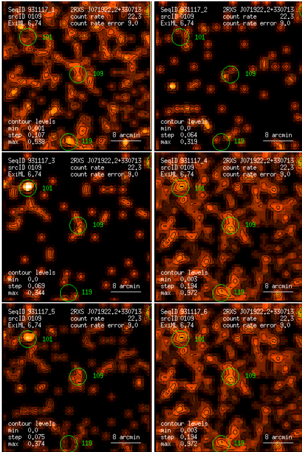
Figure 109: RASS 931117: detection 0109: band rate images, Gaussian filter: (1) PSPC channels 11 – 41, (2) 52 – 90, (3) 91 – 201, (4) 11 – 235, (5) 52 – 201, (6) 11 – 201. Broad band rates in counts/ks. Band rate contour levels in counts/ks/arcmin 2 .
