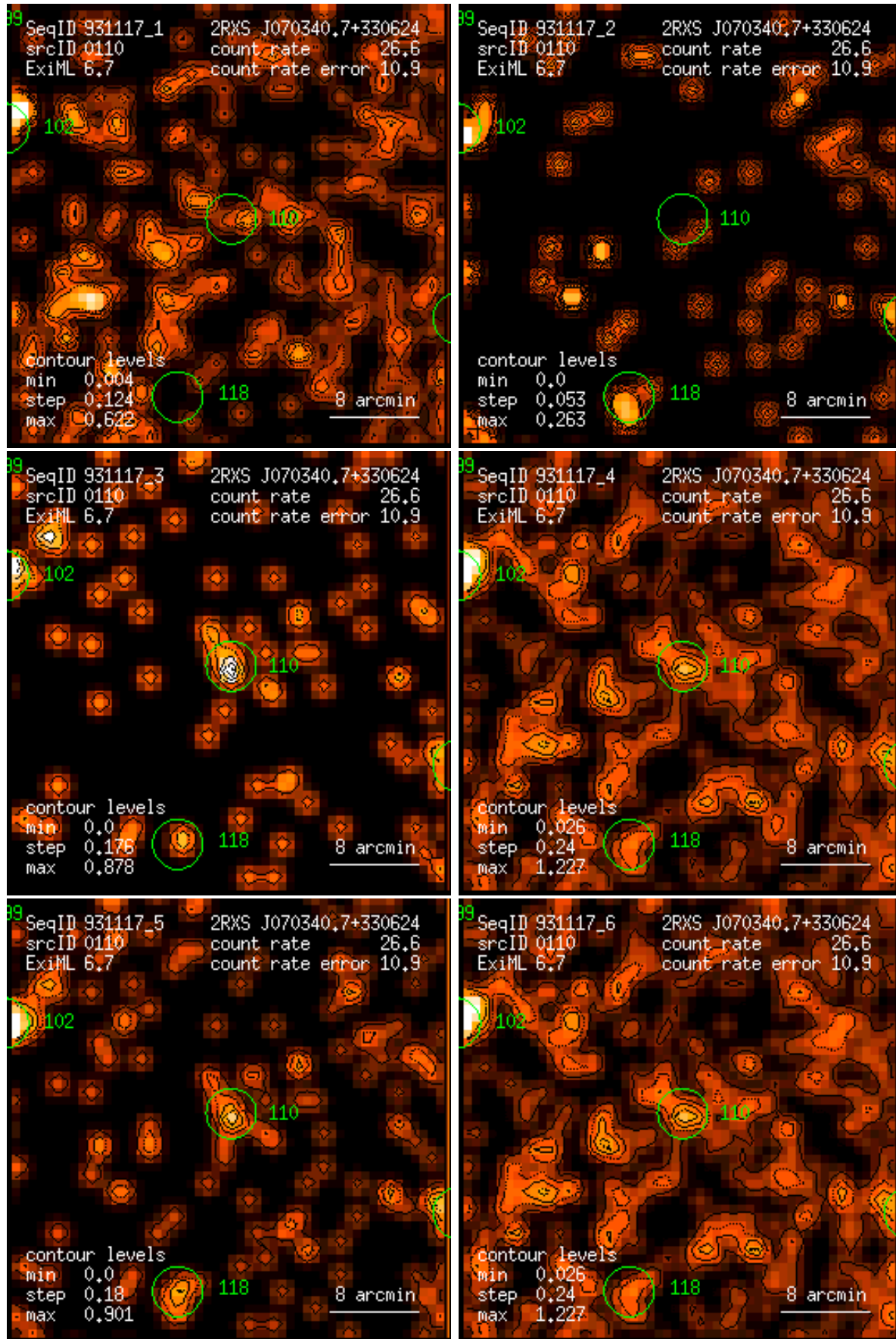
Figure 110: RASS 931117: detection 0110: band rate images, Gaussian filter: (1) PSPC channels 11 – 41, (2) 52 – 90, (3) 91 – 201, (4) 11 – 235, (5) 52 – 201, (6) 11 – 201. Broad band rates in counts/ks. Band rate contour levels in counts/ks/arcmin 2 .
