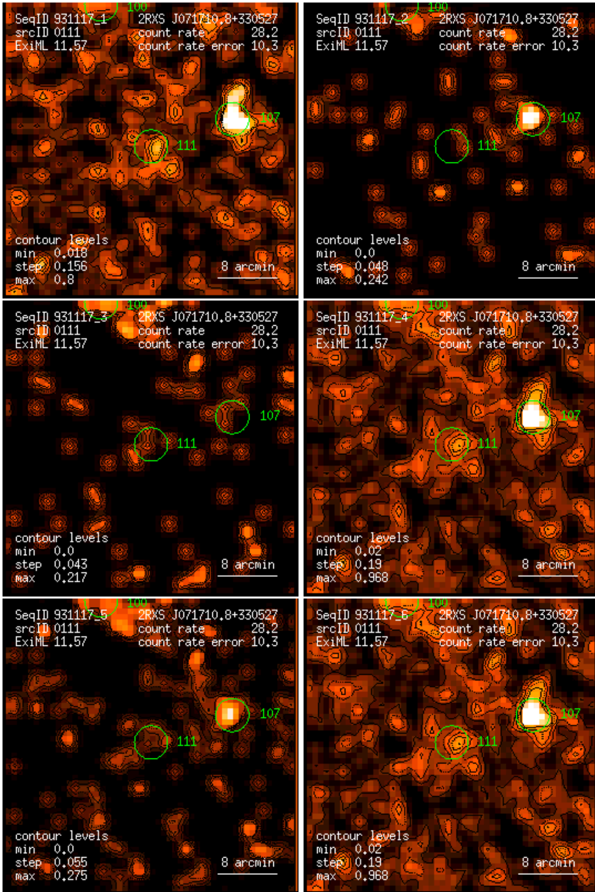
Figure 111: RASS 931117: detection 0111: band rate images, Gaussian filter: (1) PSPC channels 11 – 41, (2) 52 – 90, (3) 91 – 201, (4) 11 – 235, (5) 52 – 201, (6) 11 – 201. Broad band rates in counts/ks. Band rate contour levels in counts/ks/arcmin 2 .
