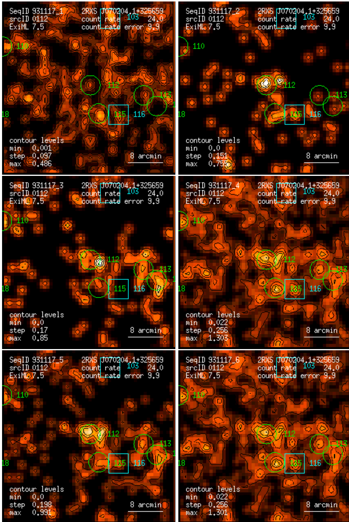
Figure 112: RASS 931117: detection 0112: band rate images, Gaussian filter: (1) PSPC channels 11 – 41, (2) 52 – 90, (3) 91 – 201, (4) 11 – 235, (5) 52 – 201, (6) 11 – 201. Broad band rates in counts/ks. Band rate contour levels in counts/ks/arcmin 2 .
