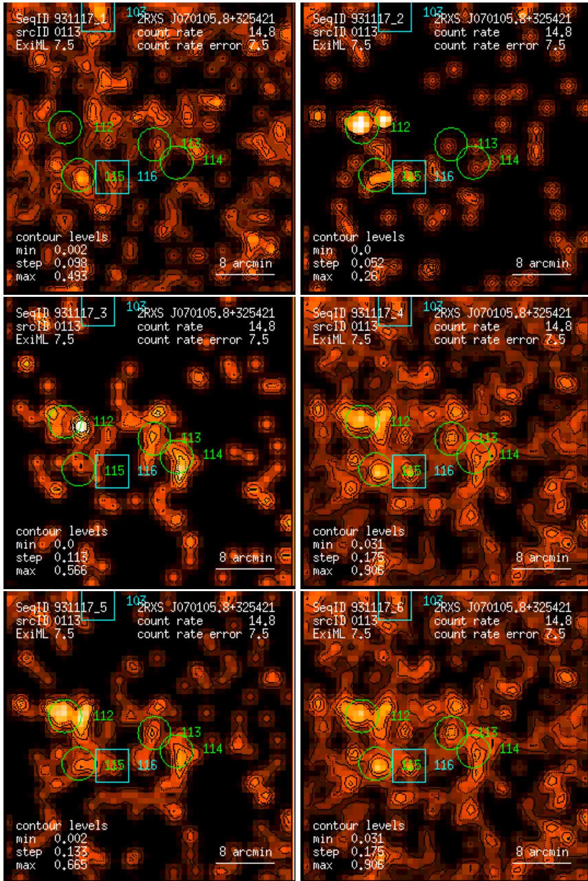
Figure 113: RASS 931117: detection 0113: band rate images, Gaussian filter: (1) PSPC channels 11 – 41, (2) 52 – 90, (3) 91 – 201, (4) 11 – 235, (5) 52 – 201, (6) 11 – 201. Broad band rates in counts/ks. Band rate contour levels in counts/ks/arcmin 2 .
