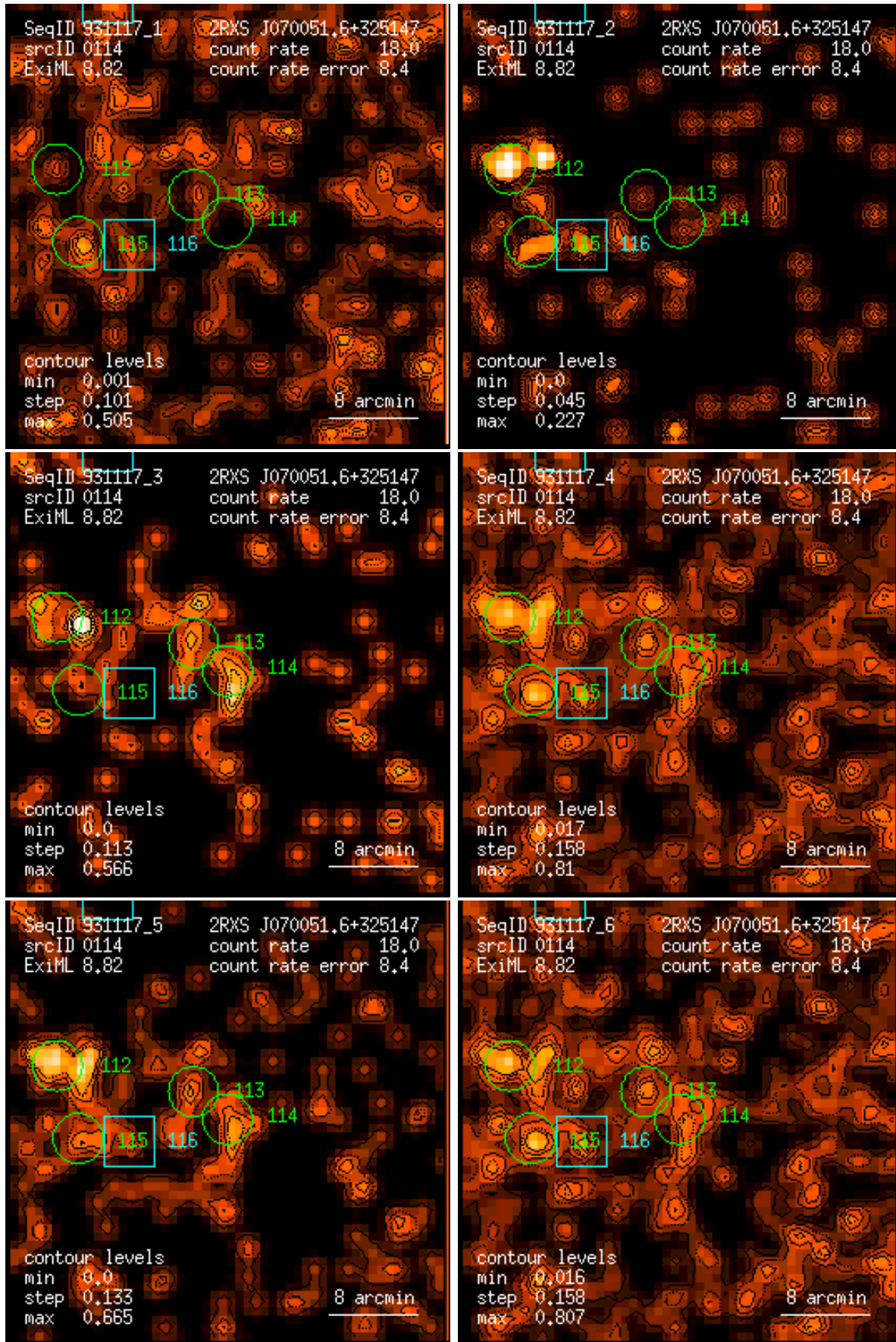
Figure 114: RASS 931117: detection 0114: band rate images, Gaussian filter: (1) PSPC channels 11 – 41, (2) 52 – 90, (3) 91 – 201, (4) 11 – 235, (5) 52 – 201, (6) 11 – 201. Broad band rates in counts/ks. Band rate contour levels in counts/ks/arcmin 2 .
