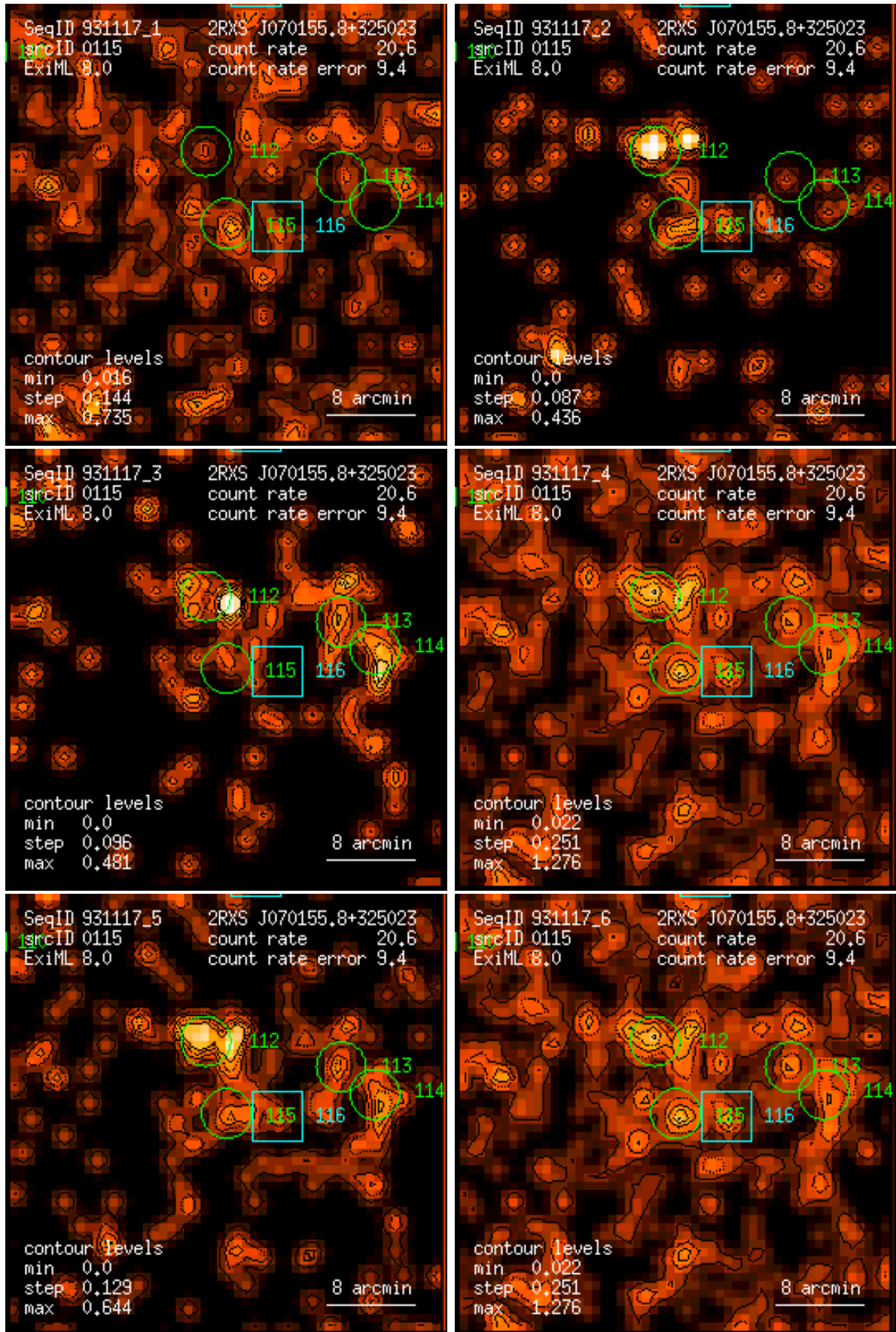
Figure 115: RASS 931117: detection 0115: band rate images, Gaussian filter: (1) PSPC channels 11 – 41, (2) 52 – 90, (3) 91 – 201, (4) 11 – 235, (5) 52 – 201, (6) 11 – 201. Broad band rates in counts/ks. Band rate contour levels in counts/ks/arcmin 2 .
