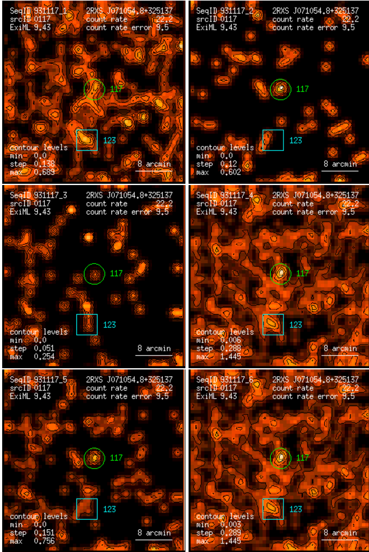
Figure 117: RASS 931117: detection 0117: band rate images, Gaussian filter: (1) PSPC channels 11 – 41, (2) 52 – 90, (3) 91 – 201, (4) 11 – 235, (5) 52 – 201, (6) 11 – 201. Broad band rates in counts/ks. Band rate contour levels in counts/ks/arcmin 2 .
