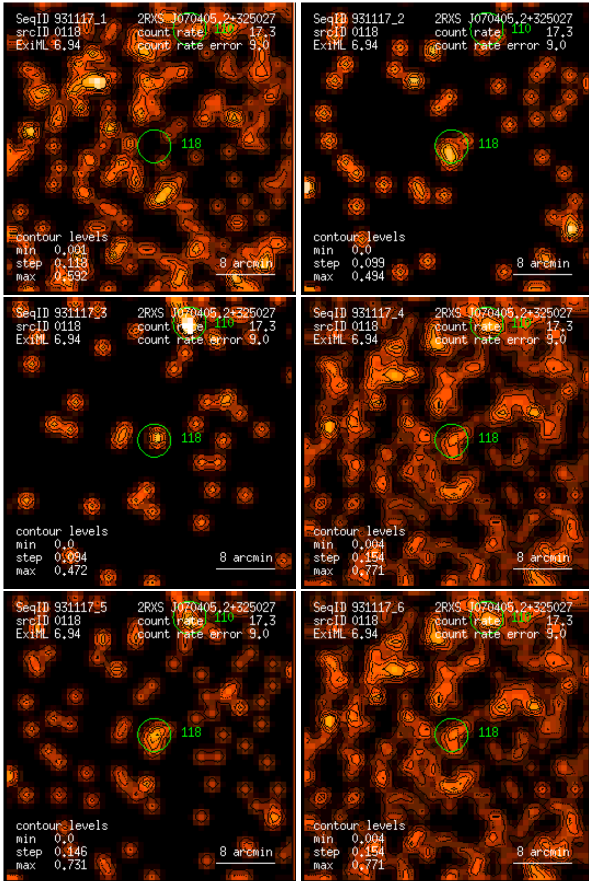
Figure 118: RASS 931117: detection 0118: band rate images, Gaussian filter: (1) PSPC channels 11 – 41, (2) 52 – 90, (3) 91 – 201, (4) 11 – 235, (5) 52 – 201, (6) 11 – 201. Broad band rates in counts/ks. Band rate contour levels in counts/ks/arcmin 2 .
