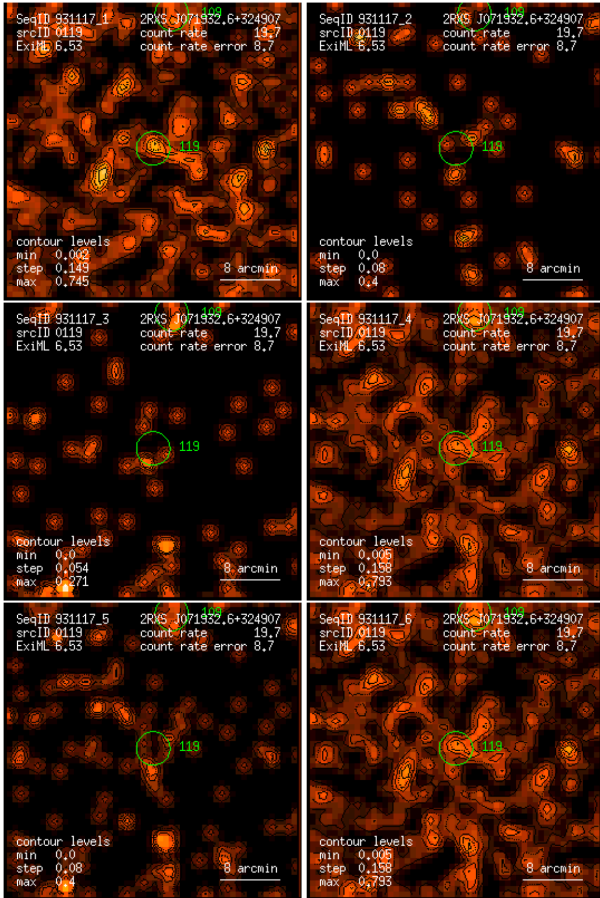
Figure 119: RASS 931117: detection 0119: band rate images, Gaussian filter: (1) PSPC channels 11 – 41, (2) 52 – 90, (3) 91 – 201, (4) 11 – 235, (5) 52 – 201, (6) 11 – 201. Broad band rates in counts/ks. Band rate contour levels in counts/ks/arcmin 2 .
