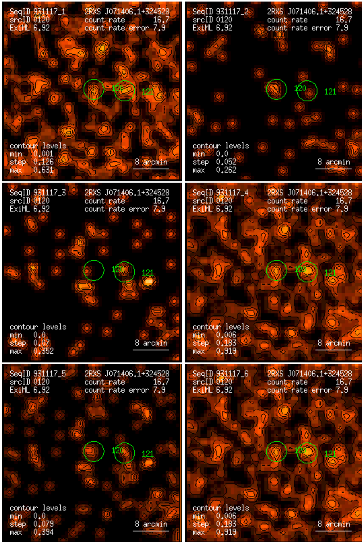
Figure 120: RASS 931117: detection 0120: band rate images, Gaussian filter: (1) PSPC channels 11 – 41, (2) 52 – 90, (3) 91 – 201, (4) 11 – 235, (5) 52 – 201, (6) 11 – 201. Broad band rates in counts/ks. Band rate contour levels in counts/ks/arcmin 2 .
