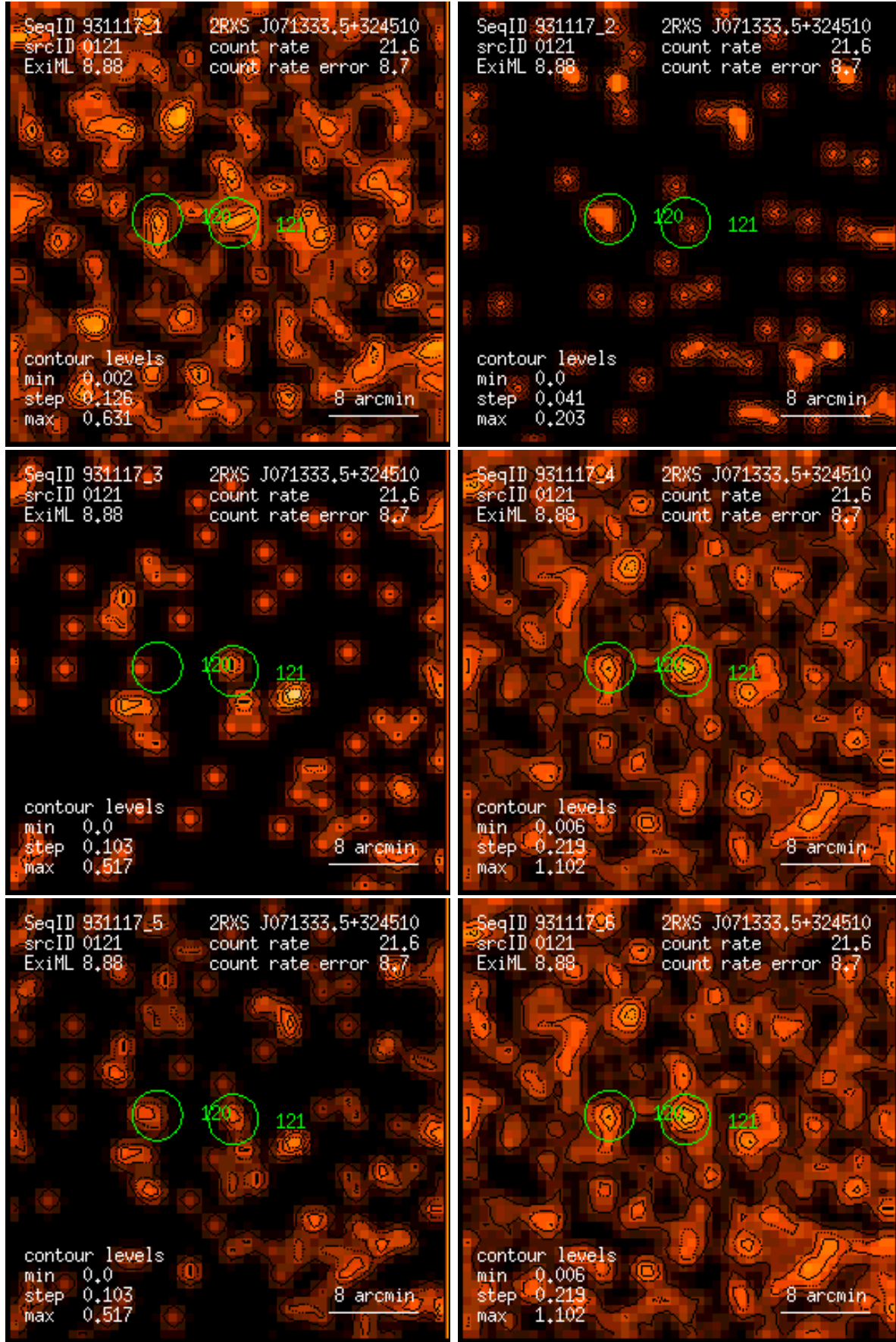
Figure 121: RASS 931117: detection 0121: band rate images, Gaussian filter: (1) PSPC channels 11 – 41, (2) 52 – 90, (3) 91 – 201, (4) 11 – 235, (5) 52 – 201, (6) 11 – 201. Broad band rates in counts/ks. Band rate contour levels in counts/ks/arcmin 2 .
