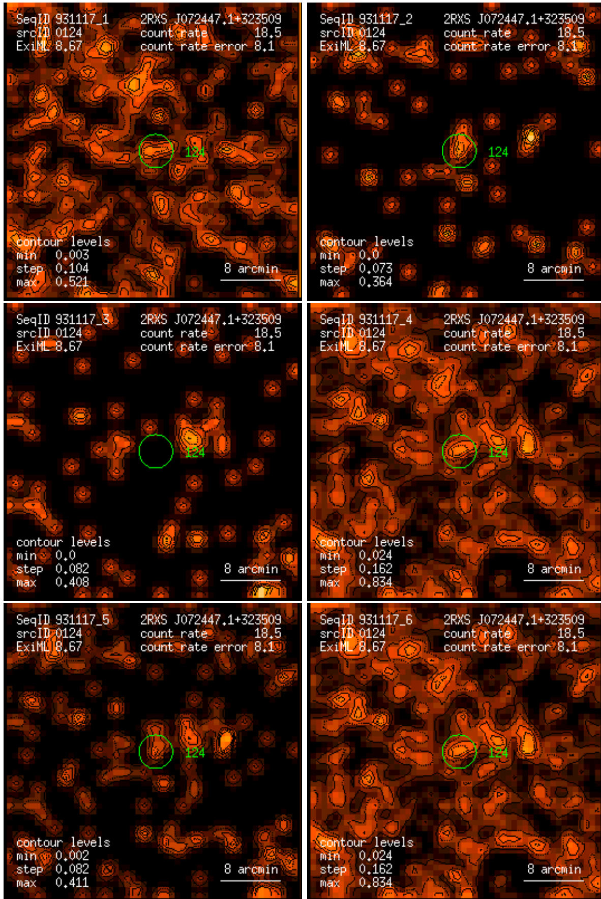
Figure 124: RASS 931117: detection 0124: band rate images, Gaussian filter: (1) PSPC channels 11 – 41, (2) 52 – 90, (3) 91 – 201, (4) 11 – 235, (5) 52 – 201, (6) 11 – 201. Broad band rates in counts/ks. Band rate contour levels in counts/ks/arcmin 2 .
