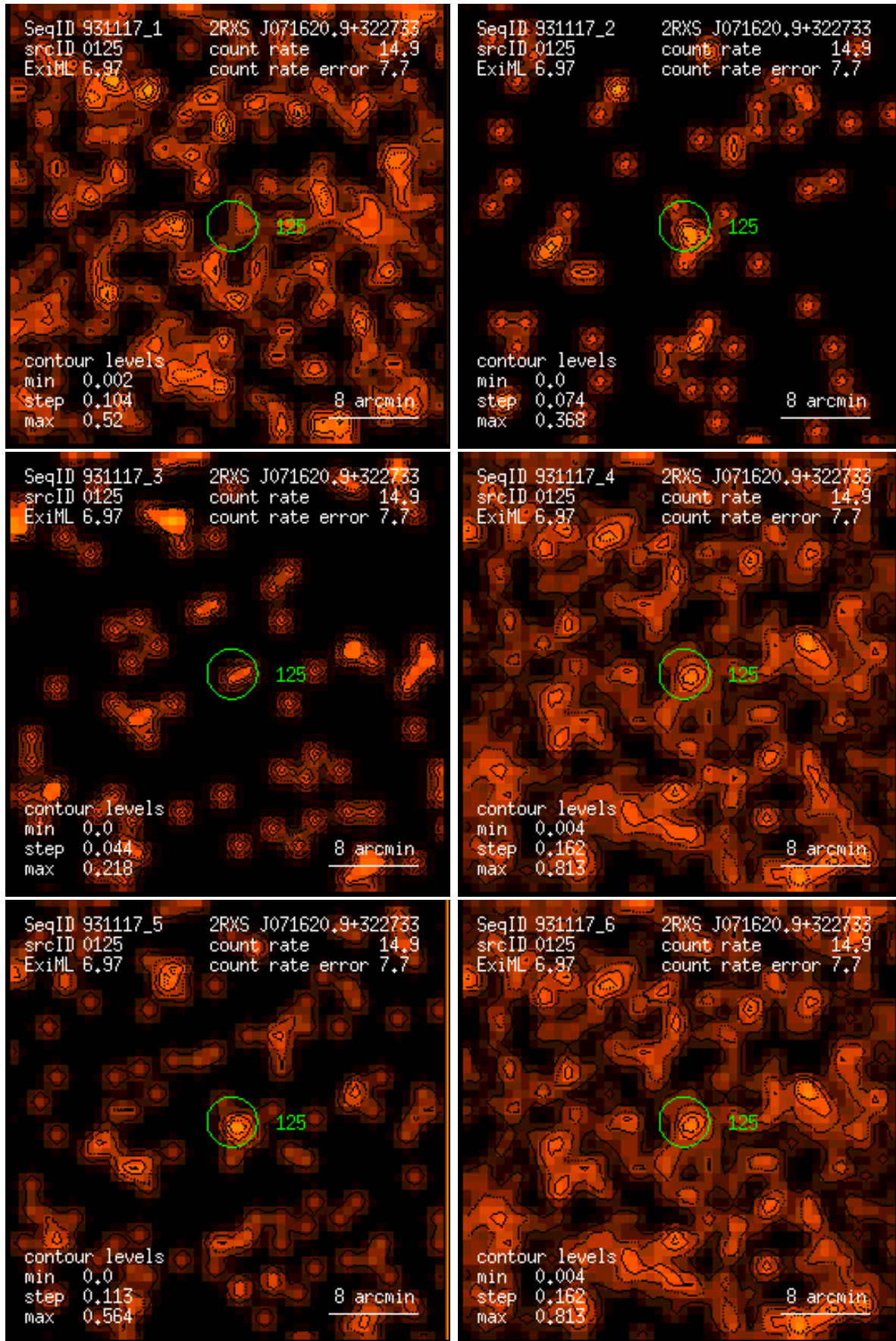
Figure 125: RASS 931117: detection 0125: band rate images, Gaussian filter: (1) PSPC channels 11 – 41, (2) 52 – 90, (3) 91 – 201, (4) 11 – 235, (5) 52 – 201, (6) 11 – 201. Broad band rates in counts/ks. Band rate contour levels in counts/ks/arcmin 2 .
