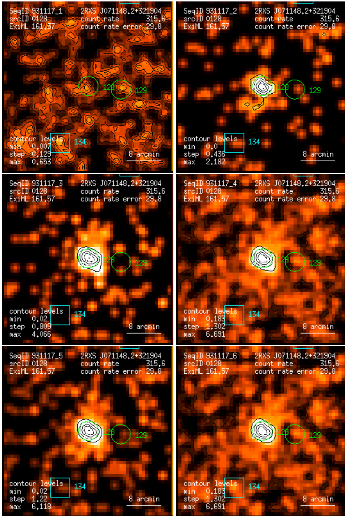
Figure 128: RASS 931117: detection 0128: band rate images, Gaussian filter: (1) PSPC channels 11 – 41, (2) 52 – 90, (3) 91 – 201, (4) 11 – 235, (5) 52 – 201, (6) 11 – 201. Broad band rates in counts/ks. Band rate contour levels in counts/ks/arcmin 2 .
