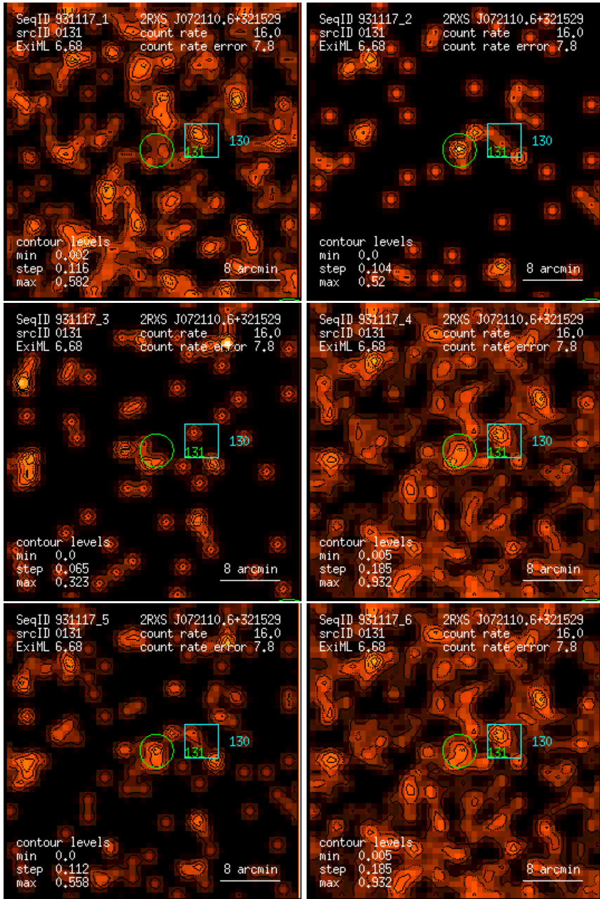
Figure 131: RASS 931117: detection 0131: band rate images, Gaussian filter: (1) PSPC channels 11 – 41, (2) 52 – 90, (3) 91 – 201, (4) 11 – 235, (5) 52 – 201, (6) 11 – 201. Broad band rates in counts/ks. Band rate contour levels in counts/ks/arcmin 2 .
