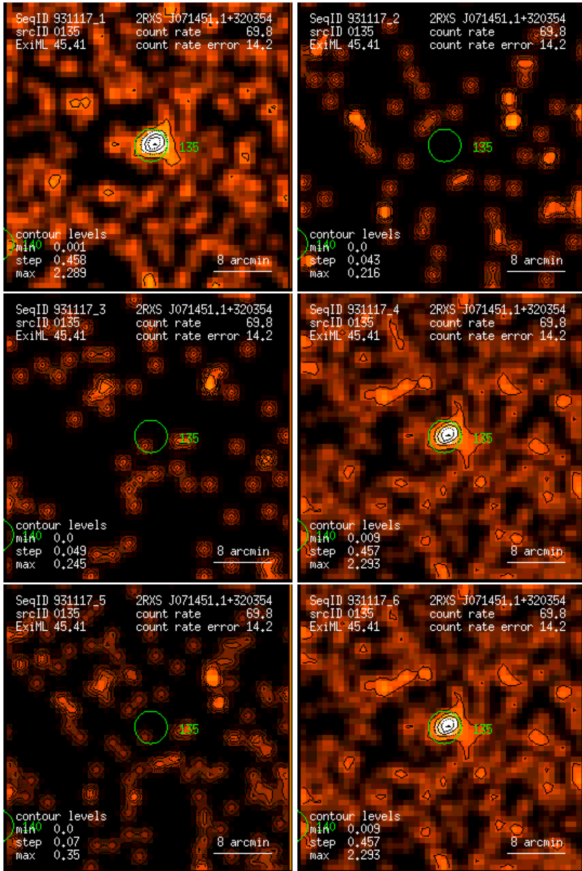
Figure 135: RASS 931117: detection 0135: band rate images, Gaussian filter: (1) PSPC channels 11 – 41, (2) 52 – 90, (3) 91 – 201, (4) 11 – 235, (5) 52 – 201, (6) 11 – 201. Broad band rates in counts/ks. Band rate contour levels in counts/ks/arcmin 2 .
