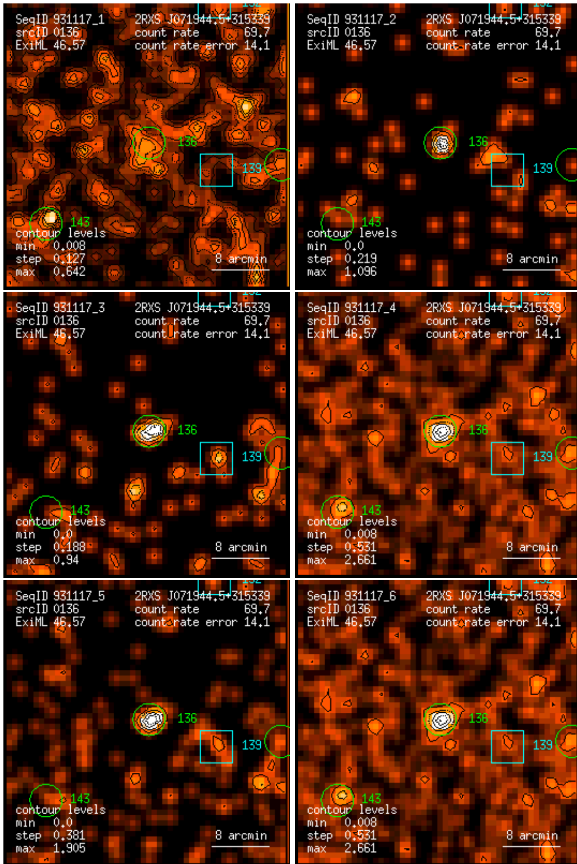
Figure 136: RASS 931117: detection 0136: band rate images, Gaussian filter: (1) PSPC channels 11 – 41, (2) 52 – 90, (3) 91 – 201, (4) 11 – 235, (5) 52 – 201, (6) 11 – 201. Broad band rates in counts/ks. Band rate contour levels in counts/ks/arcmin 2 .
