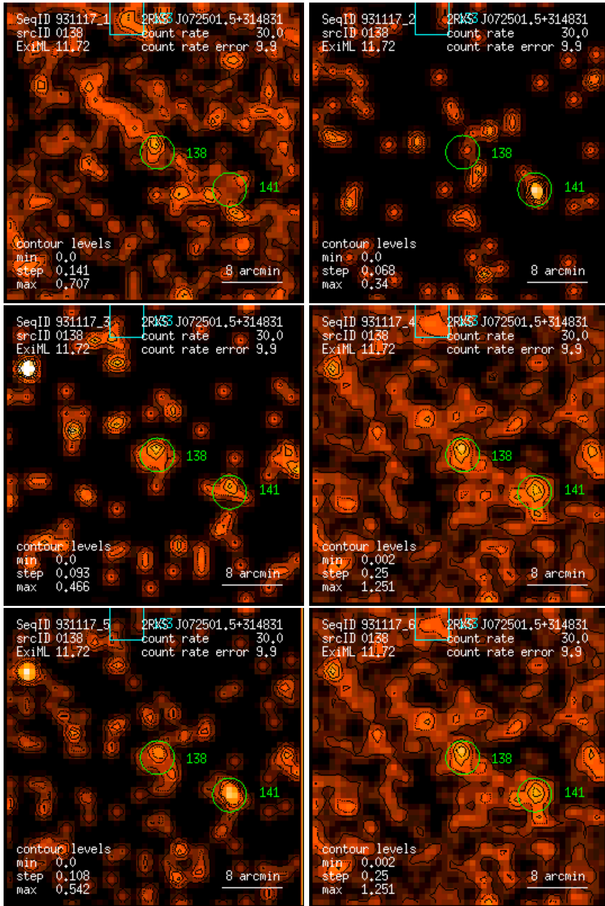
Figure 138: RASS 931117: detection 0138: band rate images, Gaussian filter: (1) PSPC channels 11 – 41, (2) 52 – 90, (3) 91 – 201, (4) 11 – 235, (5) 52 – 201, (6) 11 – 201. Broad band rates in counts/ks. Band rate contour levels in counts/ks/arcmin 2 .
