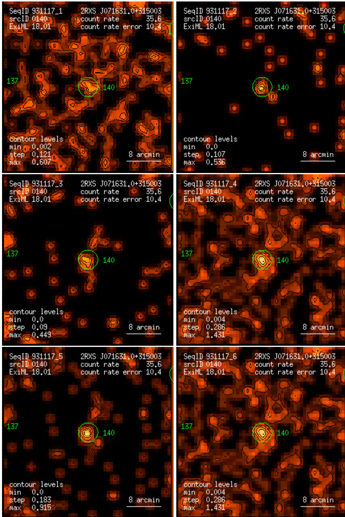
Figure 140: RASS 931117: detection 0140: band rate images, Gaussian filter: (1) PSPC channels 11 – 41, (2) 52 – 90, (3) 91 – 201, (4) 11 – 235, (5) 52 – 201, (6) 11 – 201. Broad band rates in counts/ks. Band rate contour levels in counts/ks/arcmin 2 .
