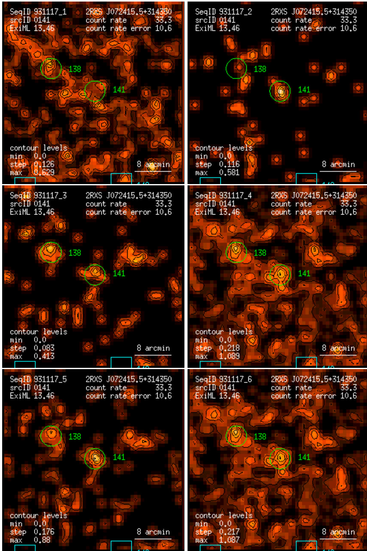
Figure 141: RASS 931117: detection 0141: band rate images, Gaussian filter: (1) PSPC channels 11 – 41, (2) 52 – 90, (3) 91 – 201, (4) 11 – 235, (5) 52 – 201, (6) 11 – 201. Broad band rates in counts/ks. Band rate contour levels in counts/ks/arcmin 2 .
