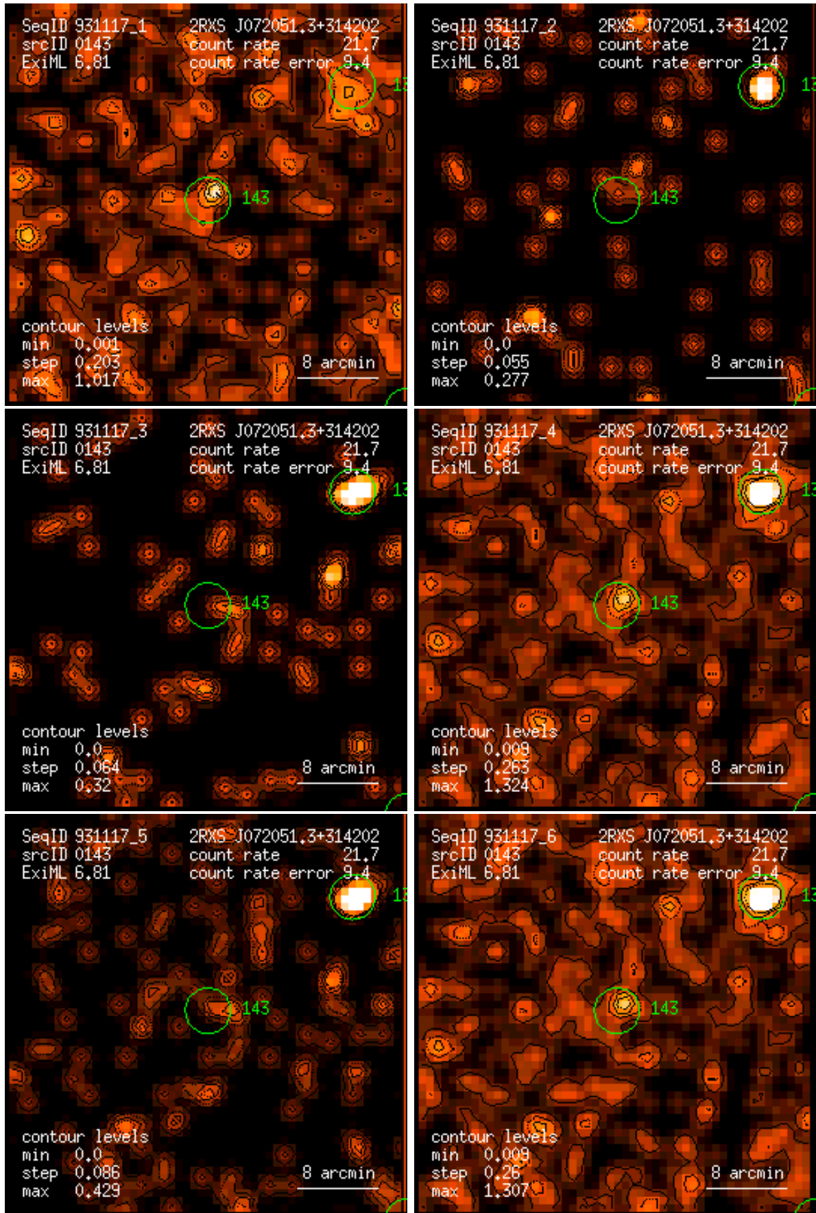
Figure 143: RASS 931117: detection 0143: band rate images, Gaussian filter: (1) PSPC channels 11 – 41, (2) 52 – 90, (3) 91 – 201, (4) 11 – 235, (5) 52 – 201, (6) 11 – 201. Broad band rates in counts/ks. Band rate contour levels in counts/ks/arcmin 2 .
